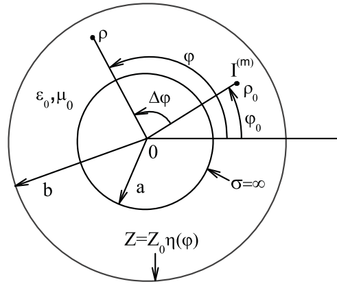
Figure 1. Azimuthal waveguide geometry.
