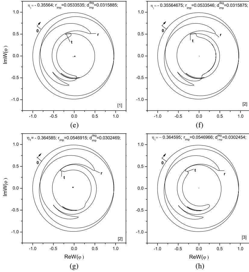
Figure 6. The normalized value of ‘diurnal record’ of the received signal W(\varphi) , ( \eta_0 = 0.1455 - 0.03638i , \eta_2 = 0.0001 , \Delta\varphi = 2 ).
