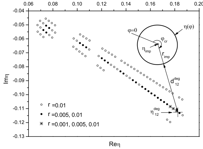
Figure 7. The domains in the complex \eta -plane, for which the CS phenomenon takes place at the given radius r_{imp} and angle \Delta\varphi = 2 .
