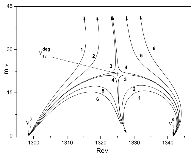
Figure 2. Trajectories of the first two roots \nu_1, \nu_2 of Equation (17) in the complex \nu -plane for several fixed values of \arg \eta_0 as |\eta_0| increases ( 0 \leq |\eta_0| \leq 0.5 ); \arg(i\eta_0) equal to (1) 63.43^\circ , (2) 60.94^\circ , (3) 58.39^\circ , (4) 58.21^\circ , (5) 55.83^\circ , (6) 53.37^\circ .
