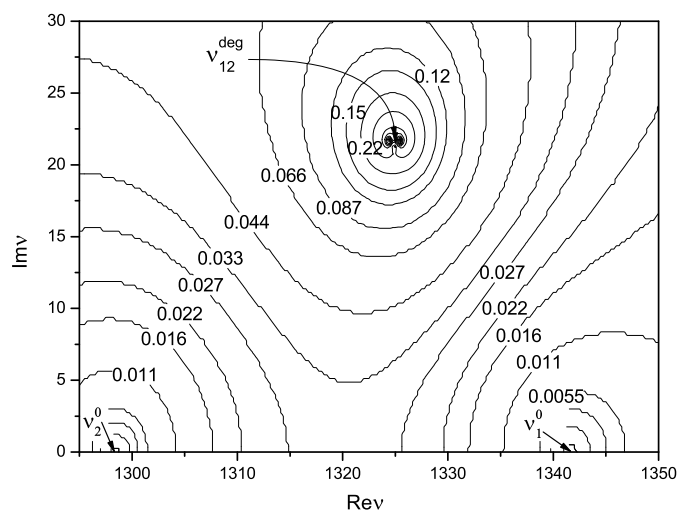
Figure 3. The level curves of the function |V_{ir}^0(\varphi_0 + \Delta\varphi, \varphi_0; \nu)| for \Delta\varphi = 2 , (\max_\nu |V_{ir}^0(\varphi_0 + 2, \varphi_0; \nu)| = 3.0517, \nu_{\max} = 1325.5 + 21.75i, |V_{ir}^0(\varphi_0 + 2, \varphi_0; \nu_1^0)| = 1.2593 \cdot 10^{-4}, |V_{ir}^0(\varphi_0 + 2, \varphi_0; \nu_2^0)| = 4.5397 \cdot 10^{-5}) .
