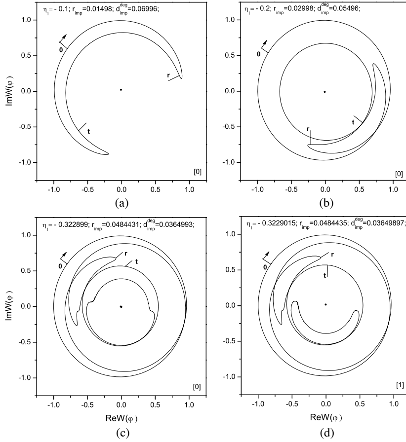
Figure 5. The normalized value of ‘diurnal record’ of the received signal W(\varphi) , ( \eta_0 = 0.1455 - 0.03638i , \eta_2 = 0.0001 , \Delta\varphi = 2 ).
