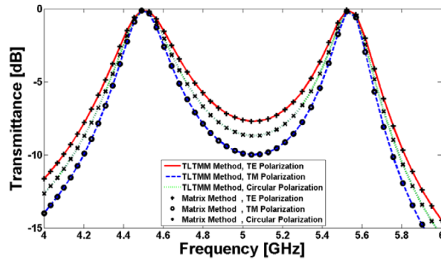
Figure 4. The transmittance-frequency dependence of a dual-band antenna radome in the C band at incident angle of 30^\circ .
