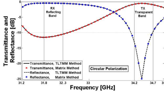
Figure 3. The transmittance and reflectance frequency responses of a dichroic plate in the Ka frequency band at incident angle of 30^\circ .
