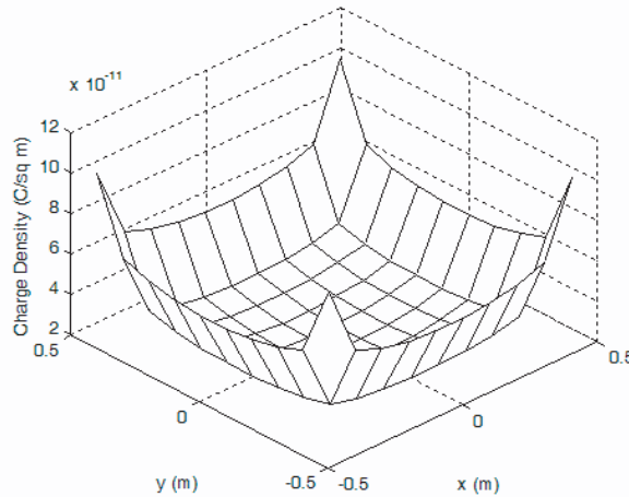
Figure 2. Charge density distribution over the plate with 100 sub domain pulse basis functions.
