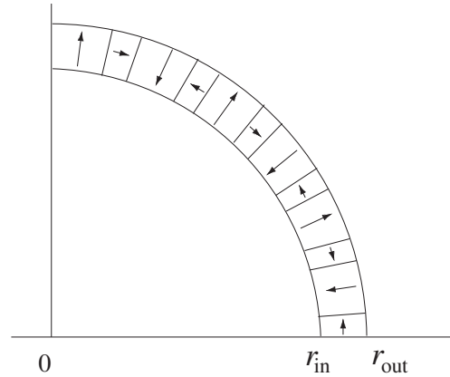
Figure 18. Representation of the optimized Halbach structure that creates a radial field whose shape is sinusoidal with the following dimensions: r = 0.024 m, r_{\text{in}} = 0.025 m, r_{\text{out}} = 0.028 m, h = 0.003 m, J = 1 T, z = 0.0015 m and 24 pairs of tile permanent magnets. The ratio between the tile permanent magnets radially and tangentially magnetized is \frac{1}{3} .
