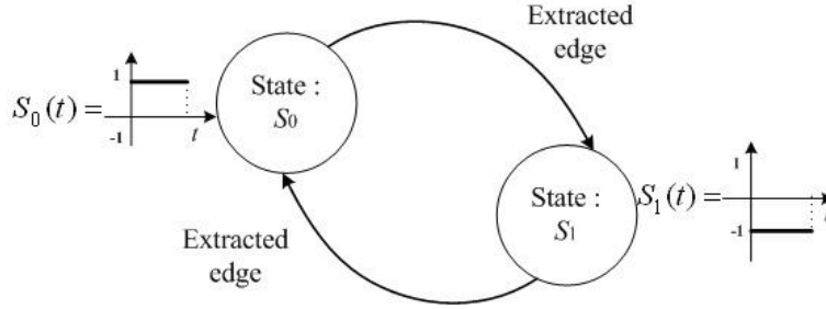
Figure 6. State diagram for generating a signal without DC-offset noise.
