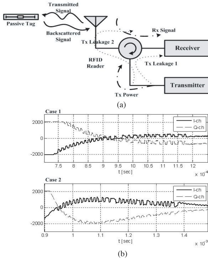
Figure 1. Description of leakage components and the corresponding DC-offset phenomenon in a passive RFID configuration.
