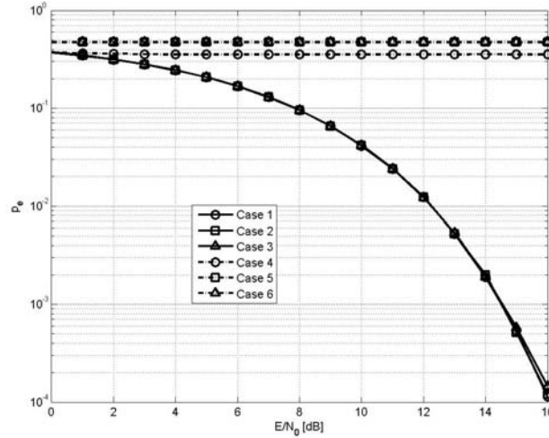
Figure 12. Comparison of the error rate performances between the traditional method and the proposed method when only the initial DC-offset value is considered for the FM0 signal with 100 symbols. Case 1: p_e vs. SNR when A_{dc} = 1.5 , B = 0 , and w_d = 0 , respectively (proposed structure). Case 2: p_e vs. SNR when A_{dc} = 5 , B = 0 , and w_d = 0 , respectively (proposed structure). Case 3: p_e vs. SNR when A_{dc} = 15 , B = 0 , and w_d = 0 , respectively (proposed structure). Case 4: p_e vs. SNR when A_{dc} = 1.5 , B = 0 , and w_d = 0 , respectively (traditional structure). Case 5: p_e vs. SNR when A_{dc} = 5 , B = 0 , and w_d = 0 , respectively (traditional structure). Case 6: p_e vs. SNR when A_{dc} = 15 , B = 0 , and w_d = 0 , respectively (traditional structure).
