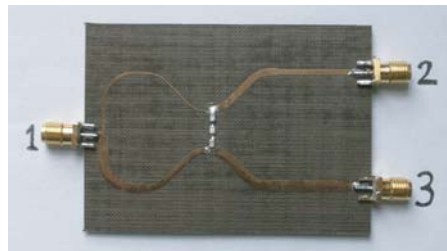
Figure 7. The fabricated unequal dual-frequency Wilkinson power divider in the second example.
