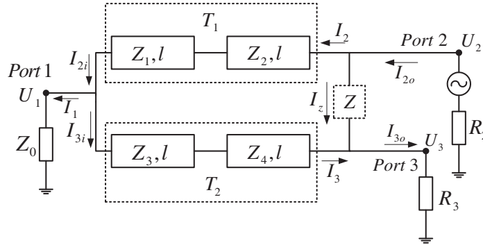
Figure 2. Equivalent circuit of the proposed power divider with voltage generator at output 2.
