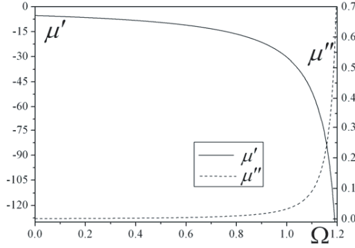
Figure 2. The frequency dispersion of the permeability \mu = \mu' + i\mu'' as a function of the non-dimensional frequency parameter \Omega = \frac{1}{2\pi} \sqrt{\varepsilon_0 \mu_0} \omega ( l = 5 \times 10^{-3} m).
