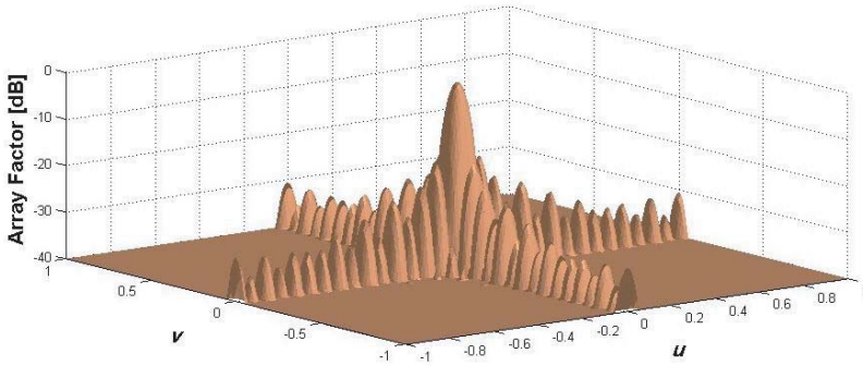
Figure 6. Array factor for the 31 \times 31 uniform element spacing planar array.
