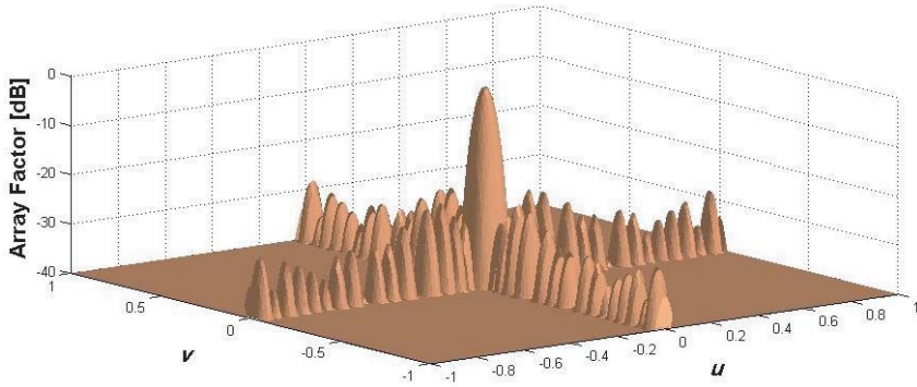
Figure 7. Array factor for the 31 \times 31 non-uniform element spacing.
