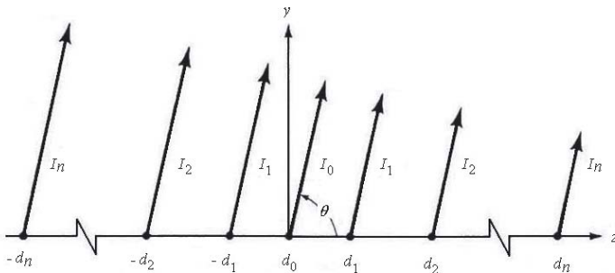
Figure 1. Geometry of 2N + 1 element no periodic symmetric linear array.
