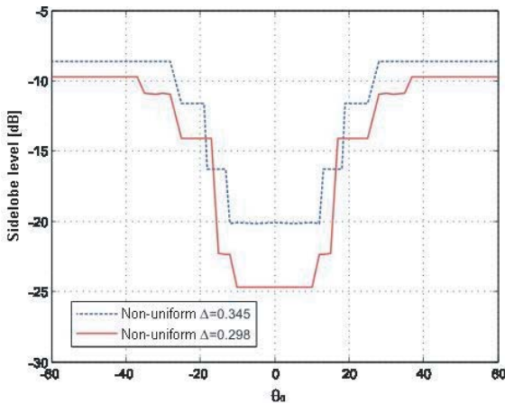
Figure 4. Sidelobe level (SLL) when the main lobe is steered in the range -60^\circ \leq \theta_0 \leq 60^\circ with non-uniform spacing in a 17 element array for different space broadening factors \Delta .
