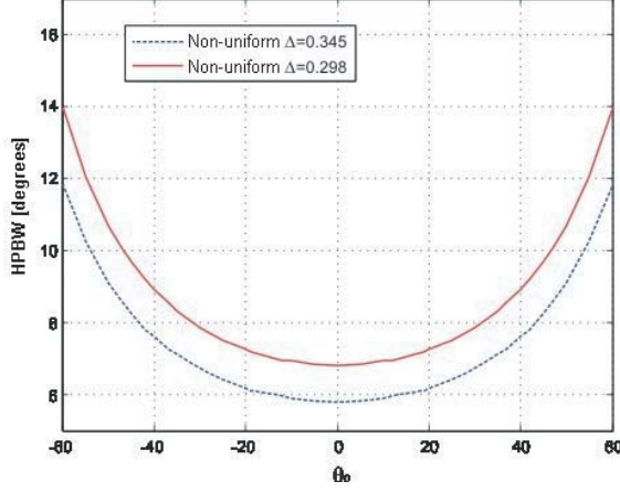
Figure 5. Half power beam width (HPBW) when the main lobe is steered in the range -60^\circ \leq \theta_0 \leq 60^\circ with non-uniform spacing in a 17 element array for different space broadening factors \Delta .
