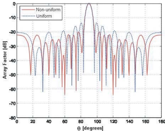
Figure 3. Array pattern for the Legendre functions synthesis with uniform (dashed line) and non-uniform spacing (solid line) of a 17 element array.
