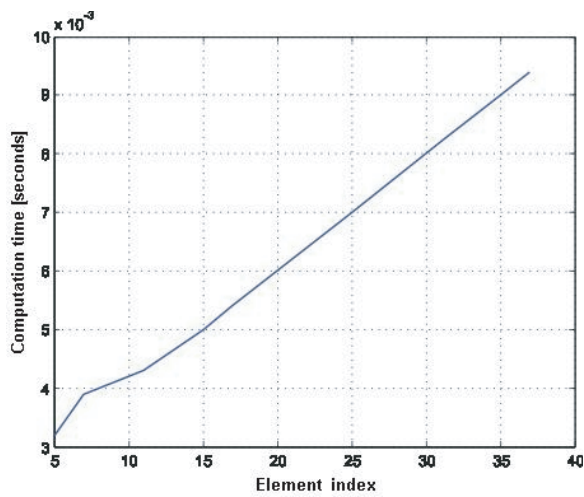
Figure 8. Computation time in a linear array applying Legendre functions.
