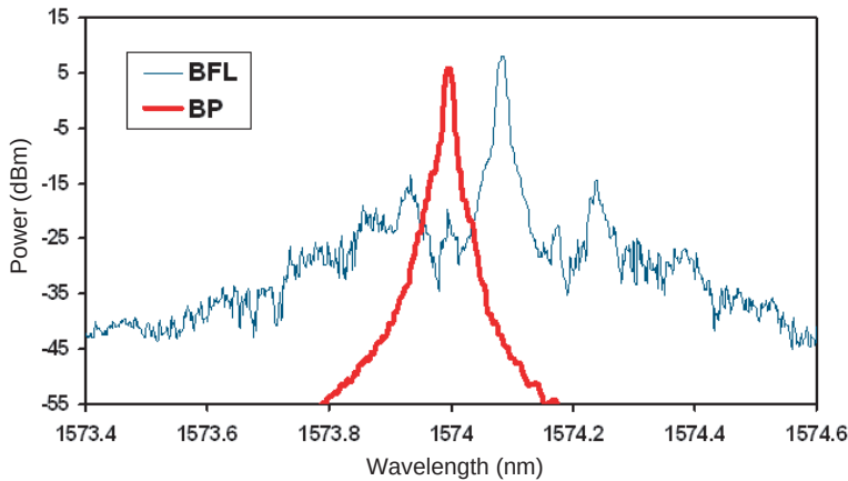
Figure 3. The input BP and BFL output spectra of the BFL.
