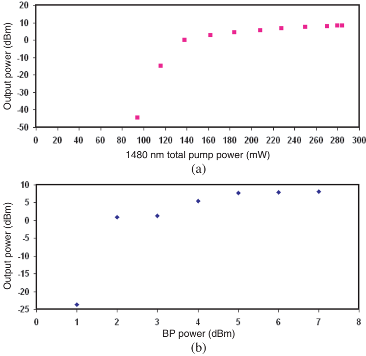
Figure 4. The peak power against the 1480 nm pump and BP powers. (a) 1480 nm pump, (b) BP.
