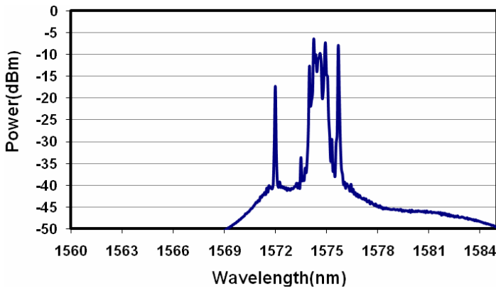
Figure 2. Free-running spectrum of the BFL.
