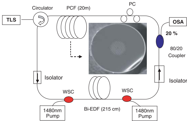
Figure 1. Configuration of the PCF-based BFL.
