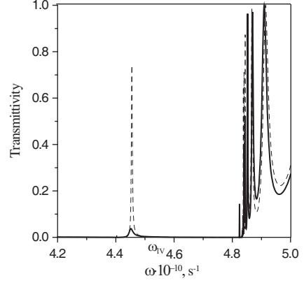
Figure 8. The frequency dependence of transmittivity ( \omega_M > \omega_{MV} , \theta = \pi/3 ): N_1 = 5 and N_2 = 8 (solid line), N_1 = 8 and N_2 = 5 (dashed line).
