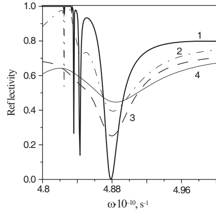
Figure 5. Reflectivity as a function of a frequency. \theta = \pi/3 , N = 5 , \omega_r = (1)0 , (2)1.06 \cdot 10^8 \text{ s}^{-1} , (3)0 , (4)1.06 \cdot 10^8 \text{ s}^{-1} , \nu = (1)0 , (2)0 , (3)10^{10} \text{ s}^{-1} , (4)10^{10} \text{ s}^{-1} .
