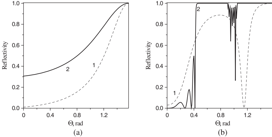
Figure 6. Reflectivity as the function of an angle of an incident wave. \omega = (a) 5 \cdot 10^{10} \text{ s}^{-1} , (b) 2 \cdot 10^{11} \text{ s}^{-1} , \varepsilon_a = \varepsilon_b = (1)1, (2)12.
