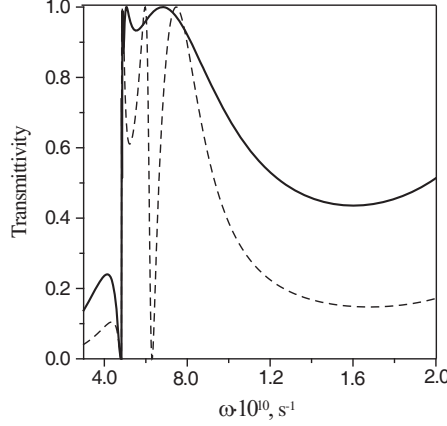
Figure 10. Transmissivity as a function of the frequency. \varepsilon_f = 5.5 , \omega_M = 3.11 \cdot 10^{10} \text{ s}^{-1} , H_0 = 2000 \text{ Oe} , \varepsilon_0 = 17.8 , \omega_p = 1 \cdot 10^{11} \text{ s}^{-1} , g = 2 , d_1 = 0.002 \text{ cm} , d_2 = 0.0005 \text{ cm} , N = 50 .
