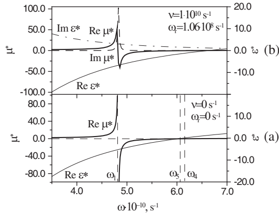
Figure 9. The frequency dependencies of the effective parameters. \varepsilon_f = 5.5 , \omega_M = 3.11 \cdot 10^{10} \text{ s}^{-1} , \varepsilon_0 = 17.8 , H_0 = 2000 \text{ Oe} , \omega_p = 1 \cdot 10^{11} \text{ s}^{-1} , g = 2 , d_1 = 0.002 \text{ cm} , d_2 = 0.0005 \text{ cm} .
