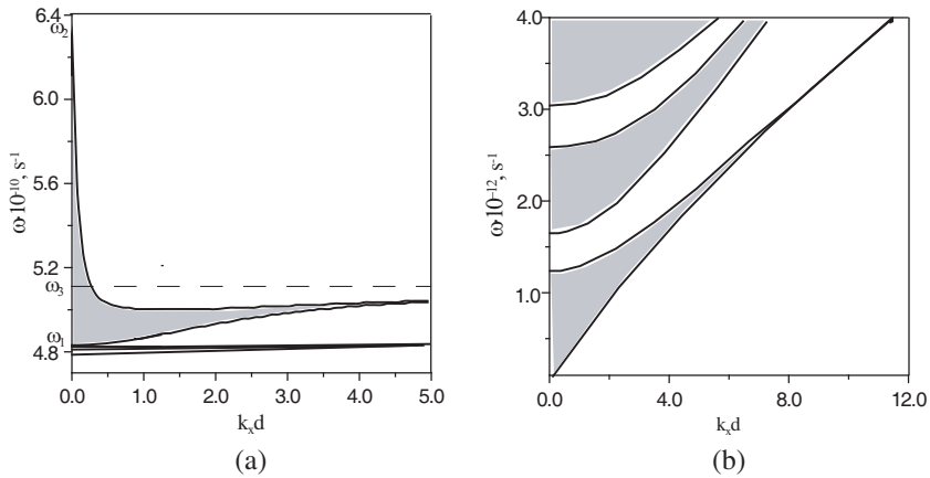
Figure 2. Dispersion dependence for the infinite structure. \varepsilon_f = 5.5 , \omega_M = 3.11 \cdot 10^{10} \text{ s}^{-1} , H_0 = 2000 \text{ Oe} , \varepsilon_0 = 17.8 , \omega_p = 1 \cdot 10^{11} \text{ s}^{-1} , g = 2 , d_1 = 0.02 \text{ cm} , d_2 = 0.005 \text{ cm} .
