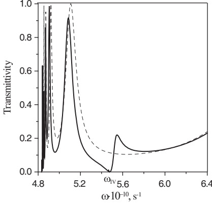
Figure 7. The frequency dependence of transmittivity, ( \omega_M < \omega_{MV} ).
