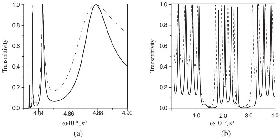
Figure 3. Transmissivity as a function of the frequency. \varepsilon_f = 5.5 , \omega_M = 3.11 \cdot 10^{10} \text{ s}^{-1} , H_0 = 2000 \text{ Oe} , \varepsilon_0 = 17.8 , \omega_p = 1 \cdot 10^{11} \text{ s}^{-1} , g = 2 , d_1 = 0.02 \text{ cm} , d_2 = 0.005 \text{ cm} .
