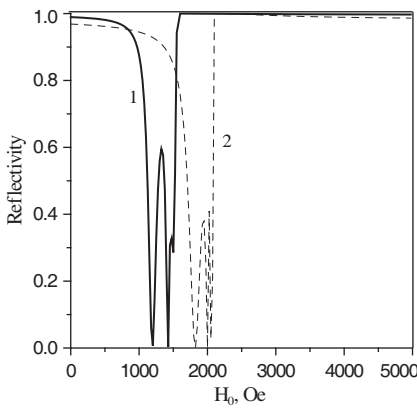
Figure 4. Reflectivity as a function of an external magnetic field ( N = 20 ).
