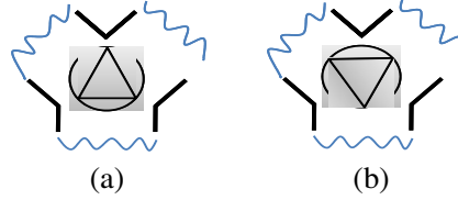
Figure 4. Geometries of two kinds of ferrite placement in the waveguide junction.
