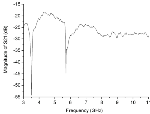
Figure 6. Measured magnitude of S_{21} .
