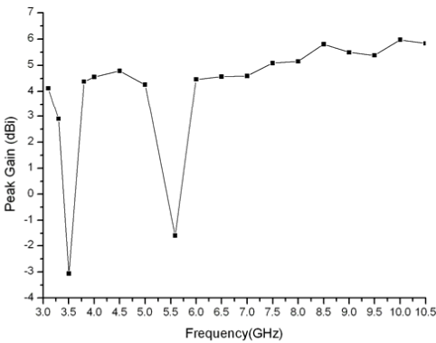
Figure 8. Measured peak gain of the proposed UWB antenna.
