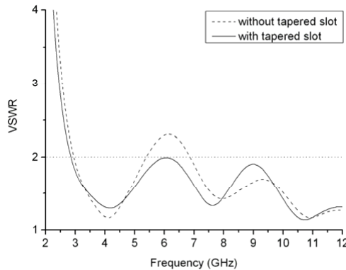
Figure 3. The comparisons of simulated VSWR results for the antennas with and without tapered slot.
