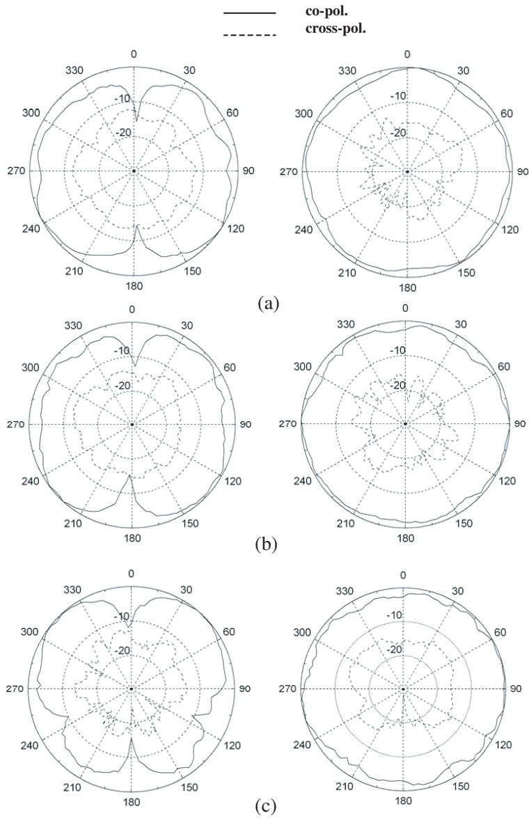
Figure 5. Measured E plane (left) and H plane (right) radiation pattern of the proposed antenna ( -10 dB/div) at (a) 3.1 GHz, (b) 4.5 GHz, (c) 7.5 GHz.
