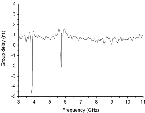
Figure 7. Measured group delay of the transfer system.
