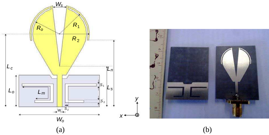
Figure 1. Configuration of the proposed antenna: (a) Geometry; (b) fabrication antenna.
