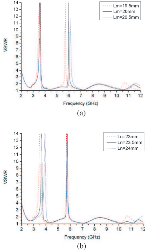
Figure 4. (a) Simulated VSWR for the proposed antenna in terms of L_m ( L_n = 23 mm); (b) simulated VSWR for the proposed antenna in terms of L_n ( L_m = 19.5 mm).
