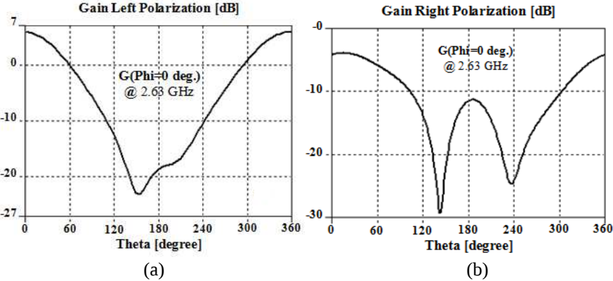
Figure 6. Gain calculated at 2.63 GHz by means of simulations performed with CST Microwave Studio for the switch configuration selecting the LHCP antenna operation mode (i.e., switches L on and switches R off).
