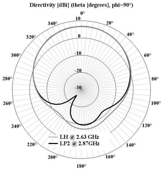
Figure 8. Directivity calculated by means of simulations performed with CST-Microwave Studio for the switch configuration selecting the LHCP and the LP2 antenna operating mode.
