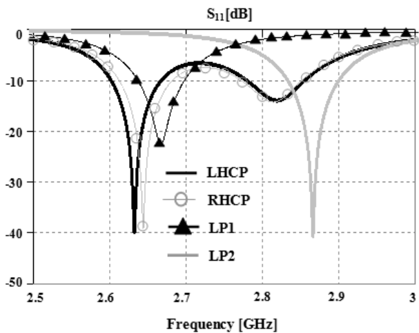
Figure 3. Measured return loss of the realized layouts corresponding to the four switch configurations illustrated in Table 1.
