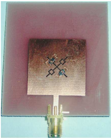
Figure 2. Realized patch antenna corresponding to the LHCP mode.
