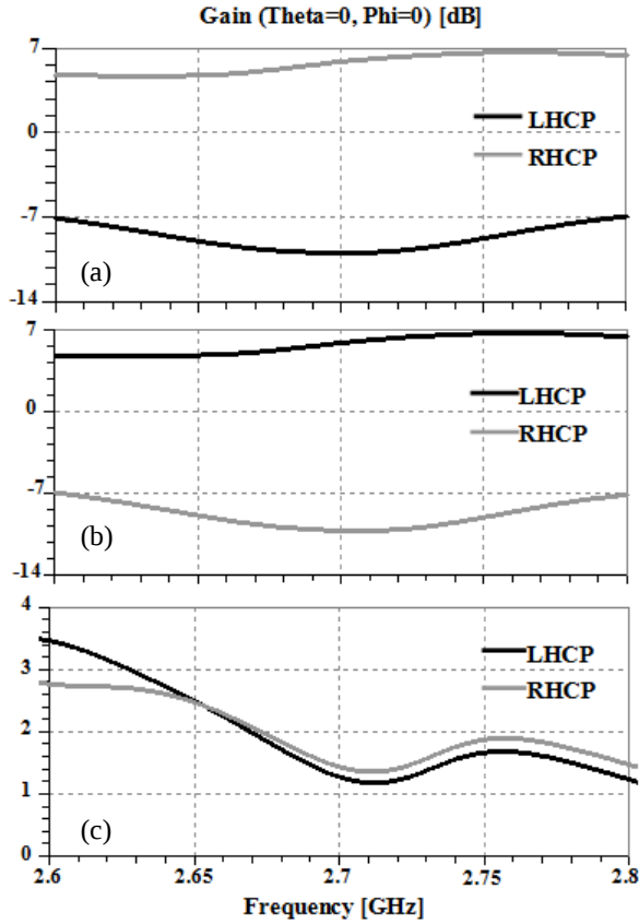
Figure 5. LHCP and RHCP Gain calculated by means of full-wave simulations: (a) switches R on and switches L off, (b) switches L on and switches R off, (c) all switches off.
