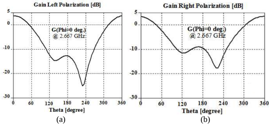
Figure 7. Gain calculated by means of simulations performed with CST Microwave Studio for the switch configuration selecting the LP antenna operation mode at 2.667 GHz (i.e., all switches off).
