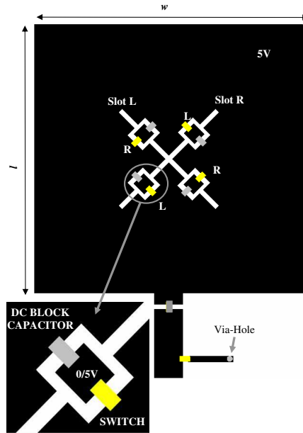
Figure 1. Geometry of the proposed antenna: a patch antenna with diagonal rectangular slots along both diagonals. Two couples ( R and L ) of switches are used to select the active slot ( L or R ).
