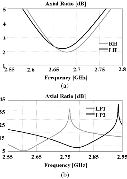
Figure 4. Axial ratio calculated by means of full-wave simulations performed with CST-Microwave studio. (a) Results obtained for the antenna in the RHCP mode (i.e., switches R on and switches L off) and in the LHCP mode (switches L on and switches R off); (b) Results obtained for the antenna in the LP1 mode (i.e., both switches R and L off) and LP2 (i.e., both switches R and L on) mode.
