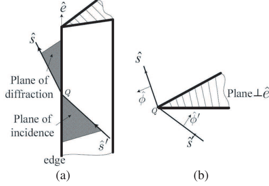
Figure 2. Sketch of the diffraction at a edge.
