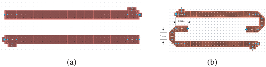
Figure 4. Parallel coupled resonators. (a) Preliminary design. (b) Modified design.
