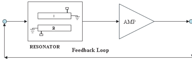
Figure 2. Basic structure of an oscillator circuit.
