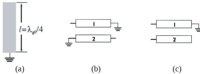
Figure 1. Quarter-wave length microstrip resonator and parallel coupled microstrip resonators.
