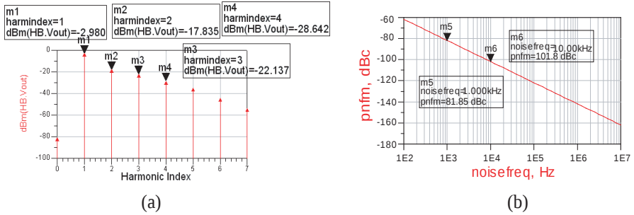
Figure 5. Power output vs harmonic index and phase noise.
