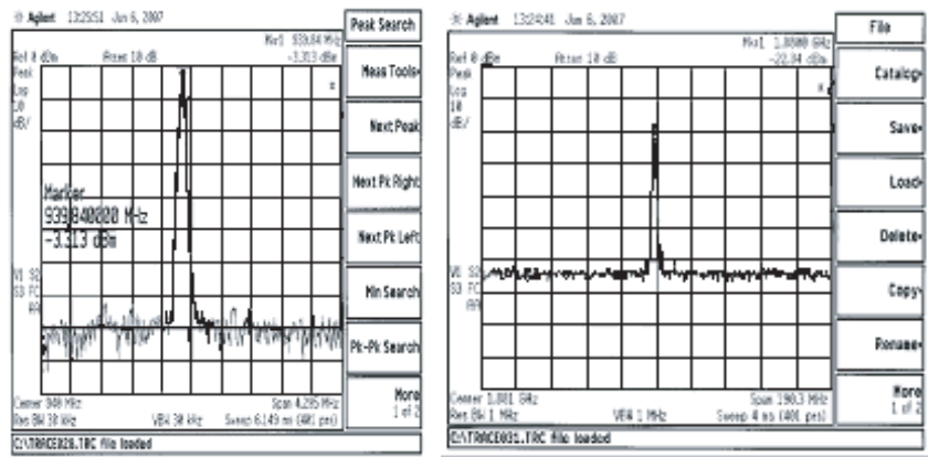
Figure 7. Fundamental frequency and second harmonic.
