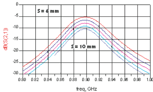
Figure 3. Bandwidth vs insertion loss.
