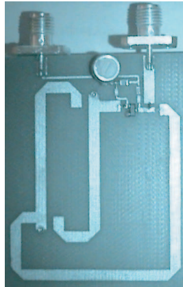
Figure 6. Fabricated oscillator.
