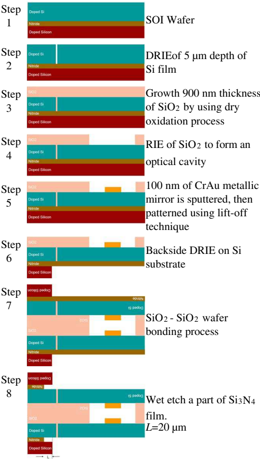
Figure 4. MEMS f-FPOTF fabrication process flow.
