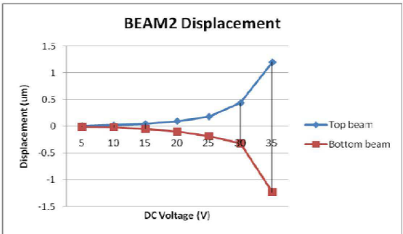
Figure 12. Displacement of BEAM2 MEMS f-FPOTF.
