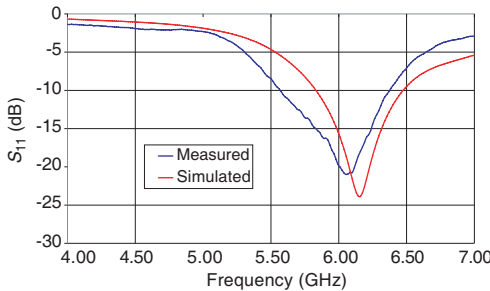
Figure 4. Measured and simulated return loss characteristics of a conventional RDRA.
