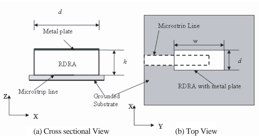
Figure 3. Geometry of the proposed compact RDRA.
