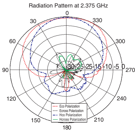
Figure 7. Measured radiation patterns for compact RDRA.
