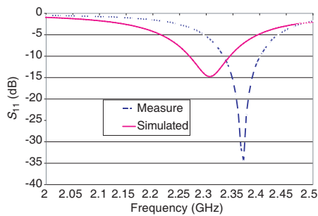
Figure 6. Measured and simulated return loss characteristics of a compact RDRA.
