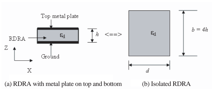
Figure 2. The compact DRA with metallic layers and its equivalent DRA in free space.
