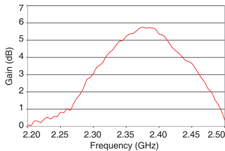
Figure 8. Measured gain for compact RDRA.
