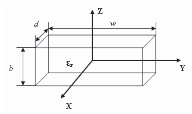
Figure 1. Geometry of an isolated rectangular dielectric resonator antenna.
