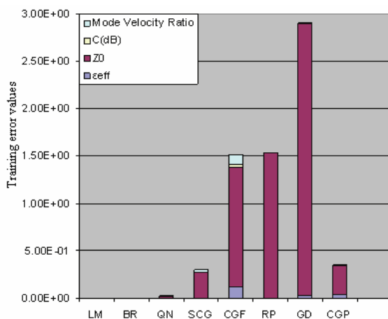
Figure 4. Bar chart comparison of training RMS error for different eight learning algorithms.
