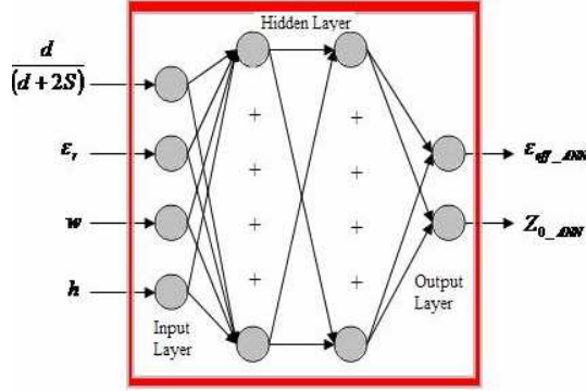
Figure 3. Configuration of proposed ANN model.
