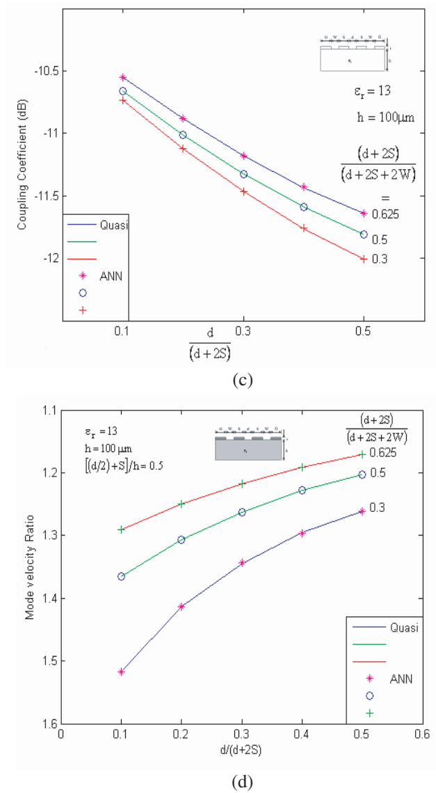
Figure 6. Comparison of CMT and neural network results of edge coupled CPW characteristics parameters, (a) effective dielectric permittivity, (b) odd & even-mode characteristics impedance, (c) coupling coefficient and (d) mode-velocity ratio.
