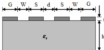
Figure 1. Cross section of edge coupled coplanar waveguides.
