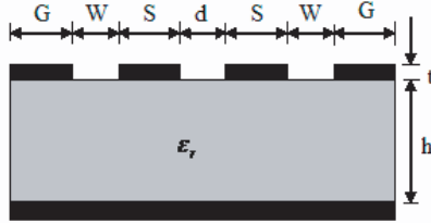
Figure 2. Cross section of conductor-backed edge-coupled CPW.
