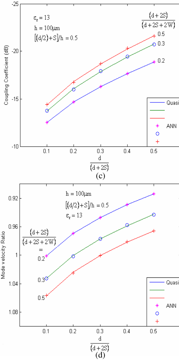
Figure 7. Comparison of CMT and neural network results of edge coupled conductor-backed CPW characteristics parameters, (a) effective dielectric permittivity, (b) odd & even-mode characteristics impedance, (c) coupling-coefficient and (d) mode-velocity ratio.
