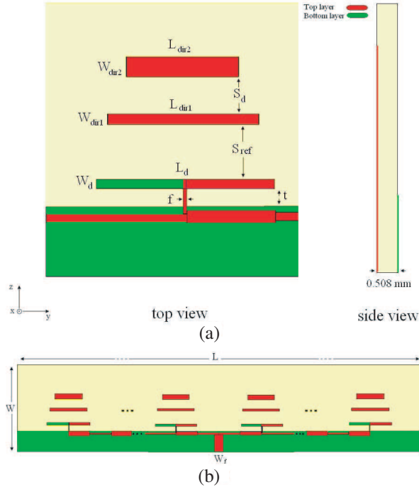
Figure 1. Series fed printed Yagi-like antenna array. (a) The single antenna element (b) The antenna array details.
