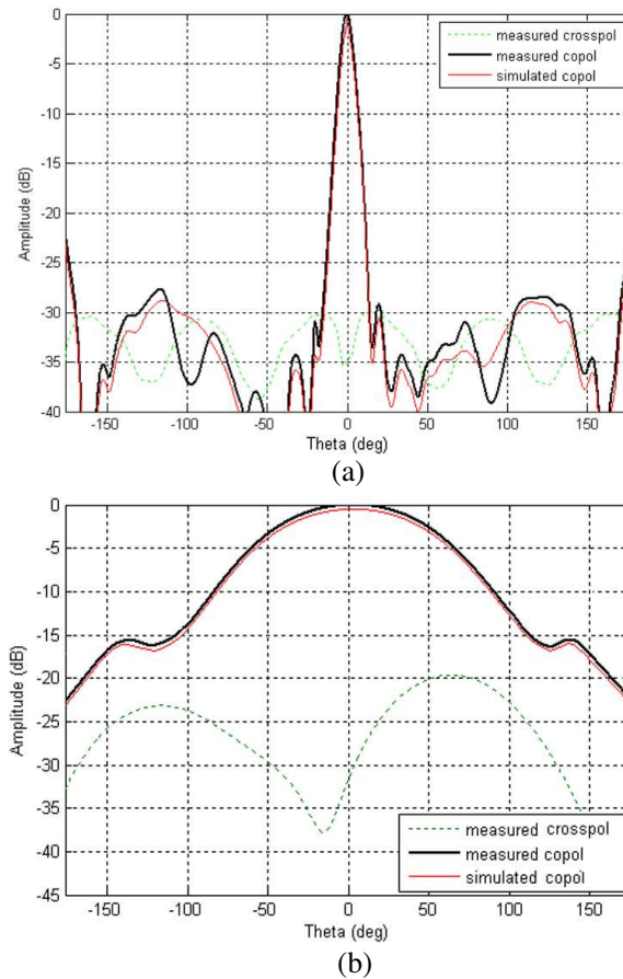
Figure 4. The simulated and measured radiation patterns of the SFY antenna array in the (a) ( y - z ) plane and (b) ( x - z ) plane.
