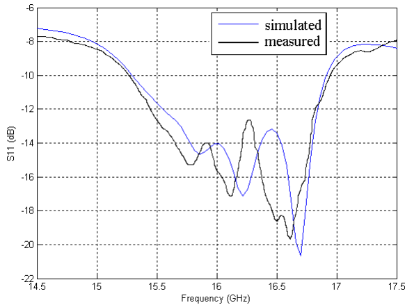
Figure 5. The simulated and measured reflection coefficient of the modified series fed Yagi-like antenna array, MSFY.
