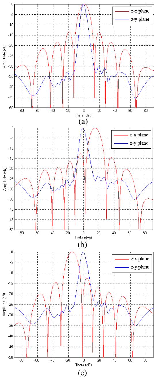
Figure 8. The simulated radiation pattern of the phased array of MSFY antenna array. Scanning angle of (a) 0^\circ , (b) +16^\circ , (c) -16^\circ .
