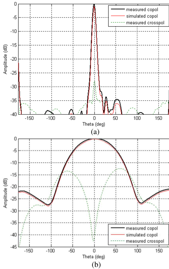
Figure 6. The simulated and measured far field radiation patterns of the MSFY antenna array at centre frequency. (a) ( y - z ) plane, (b) ( x - z ) plane.
