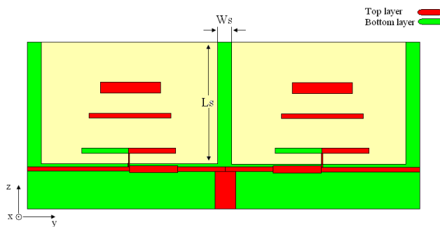
Figure 2. The center elements of the Modified series fed Yagi-like antenna array, MSFY.
