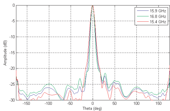
Figure 7. The simulated ( y - z ) plane radiation pattern of the MSFY antenna array at three different frequencies over the bandwidth.
