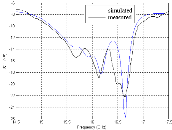
Figure 3. Simulated and Measured reflection coefficient of the SFY antenna array.
