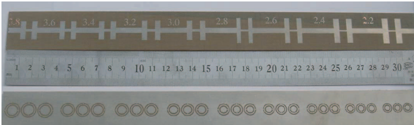
Figure 4. The photo of proposed CSF based on 9-DGS LPF. (Up: top view, middle: ruler, down: bottom view).
