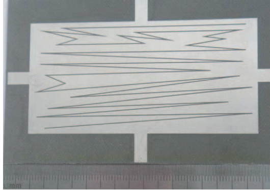
Figure 8. The photo of the proposed CSF based on the random microwave structure.
