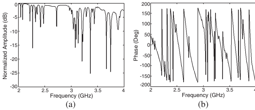
Figure 9. (a) The amplitude-frequency response and (b) the phase-frequency response of developed CSF shown in Fig. 8.
