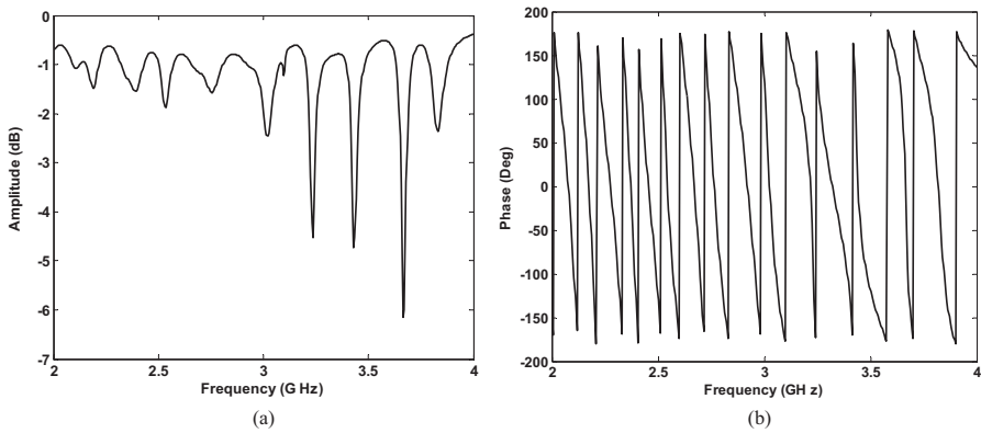
Figure 5. (a) The amplitude-frequency response and (b) the phase-frequency response.
