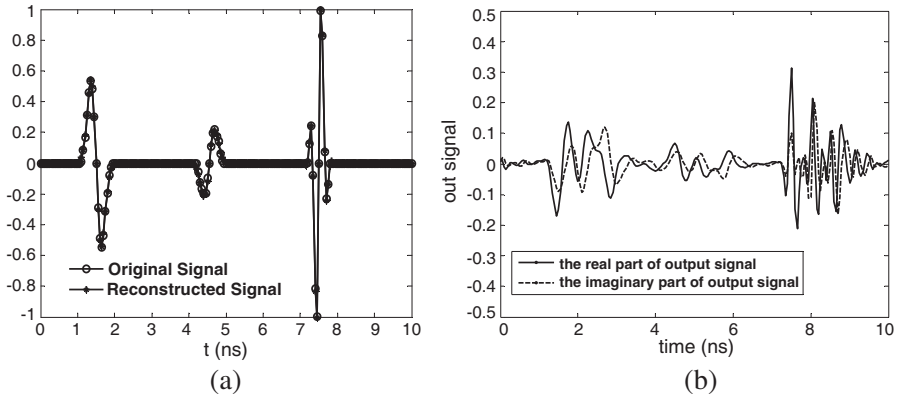
Figure 7. (a) The original and reconstructed signal, (b) the real and imaginary part of output signal.
