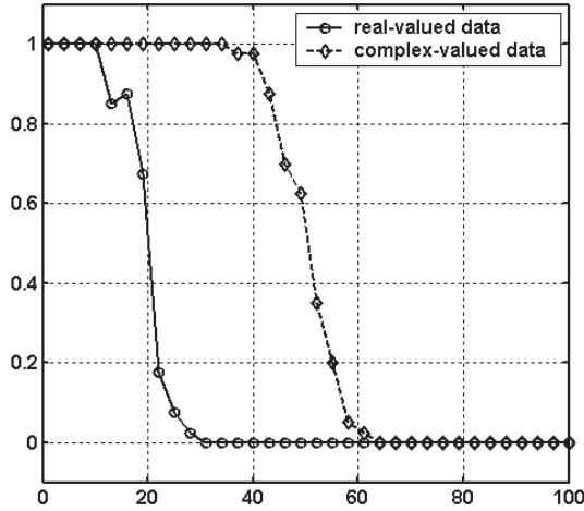
Figure 13. Probability of success of proposed SAW-CSF in the recovery of the sparest signal when the dimension of unknown signal is 200 and measurements (complex data represented by dashed line and real data represented by solid line) are 50, where x -axis denotes the cardinality of the solution, y -axis denotes the probability of success.
