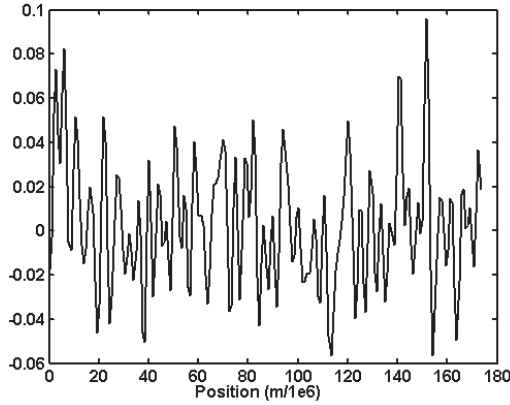
Figure 11. The curve w(x) .
