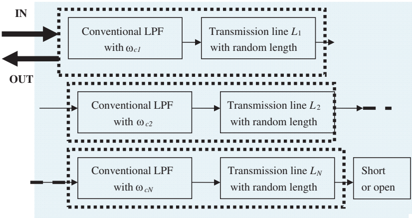
Figure 3. The scheme map of the compressive sensing filter by LPF.
