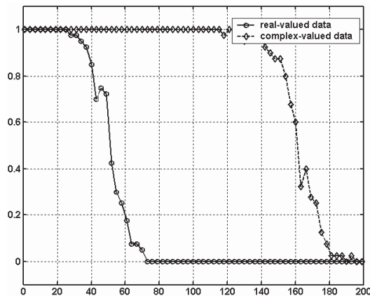
Figure 10. Probability of success of developed CSF shown in Fig. 8 in the recovery of the sparsest signal when the length of unknown signal is 400 and 1/3-Nyquist measurements (the complex data represented by the dashed line and the real data represented by the solid line), where x -axis denotes the cardinality of the solution, y -axis denotes the probability of success.
