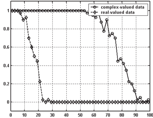
Figure 6. Probability of success of developed CSF shown in Fig. 4 in the recovery of the sparsest signal when the dimension of unknown signal is 200 and measurements (the complex data represented by solid line and the real data represented by dashed line) are 66, where x -axis denotes the cardinality of the solution, y -axis denotes the probability of success.
