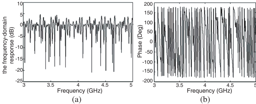
Figure 12. The simulated frequency-domain response of proposed CSF based on SAW (a) the amplitude-frequency response, (b) the phase-frequency response.
