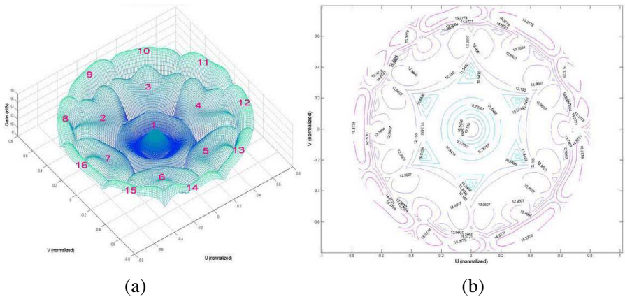
Figure 4. The simulation results: (a) 3D plots; (b) contour map.
