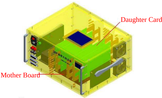
Figure 8. Interconnection structure of BFN hardware platform.
