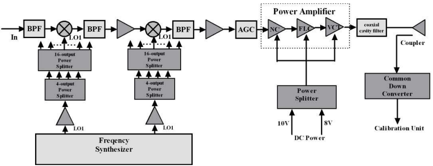
Figure 5. Block diagram of TX module.
