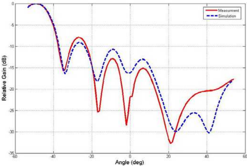
Figure 15. The elevation plane pattern of one beam in the third circle.
