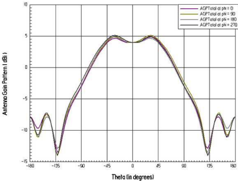
Figure 3. The simulated result of antenna element's radiation pattern.
