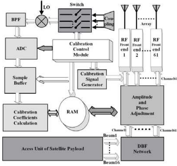
Figure 10. Block diagram of calibration unit.
