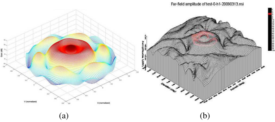
Figure 12. Three-dimensional radiation pattern of main beam: (a) simulation results; (b) measurements.
