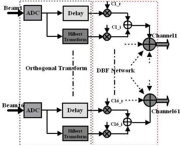
Figure 7. Block diagram of digital BFN.
