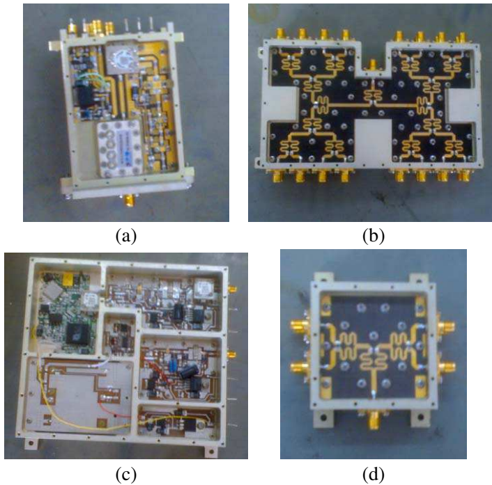
Figure 6. Photograph of subunits in RF front end: (a) TX module; (b) 16-output power splitter network; (c) frequency synthesizer; (d) 4-output power splitter network.
