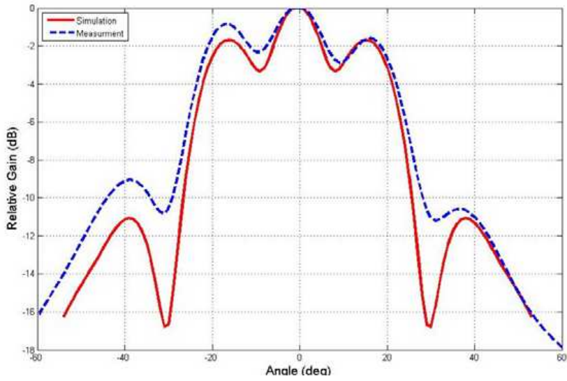
Figure 13. The elevation plane pattern of main beam (normalized).
