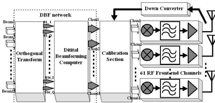
Figure 1. Block diagram of DBF transmitter antenna.
