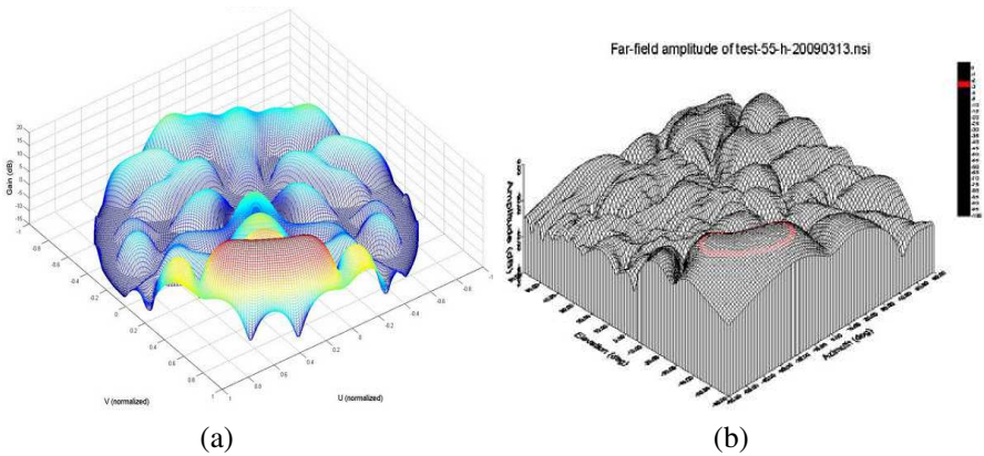
Figure 14. Three-dimensional radiation pattern of one beam in the third circle: (a) simulation results; (b) measurements.
