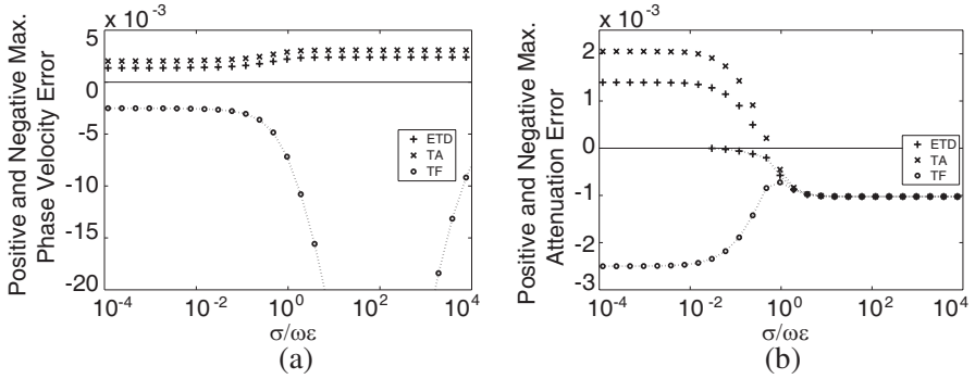
Figure 5. Same as Fig. 3, but for \sigma^*/\omega\mu = 10^2 .
