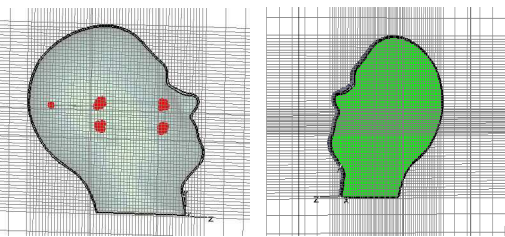
Figure 3. Mesh view for two cut planes of the complete model showing the nonuniform meshing scheme adopted for simulation.
