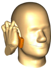
Figure 1. Complete model used for simulation including handset and SAM phantom head.
