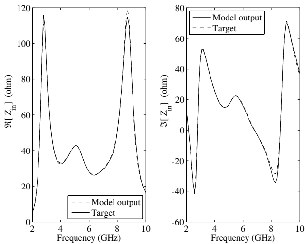
Figure 5. \Re[Z_{in}] and \Im[Z_{in}] against frequency corresponding to test geometry of Fig. 4.
