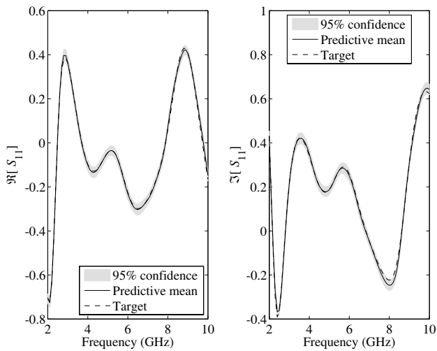
Figure 4. \Re[S_{11}] and \Im[S_{11}] against frequency for UWB test geometry [a, b, c, d, e] = [9.57, 10.75, 1.54, 2.37, 1.38] mm.
