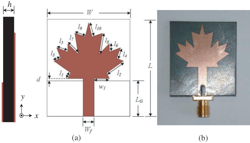
Figure 1. (a) Geometry of the proposed maple-leaf shaped printed monopole antenna. (b) Photograph of the proposed antenna prototype.
