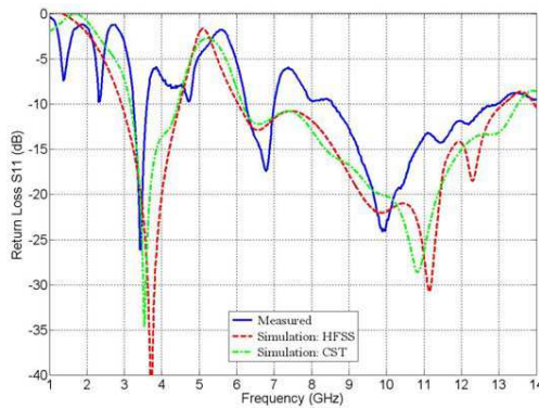
Figure 6. Measured and simulated reflection coefficient curves for the proposed bandstop antenna using an H-slot.
