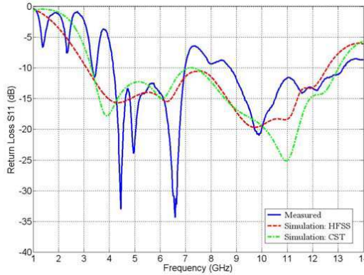
Figure 2. Measured and simulated reflection coefficient curves versus frequency of the proposed maple-leaf shaped printed monopole antenna.
