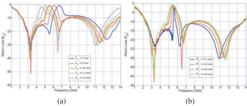
Figure 8. Simulated reflection coefficient curves for different (a) slit lengths L_S with W_S = 0.5 mm and S = 3 mm, (b) slit widths W_S with L_S = 10.2 mm and S = 3 mm.
