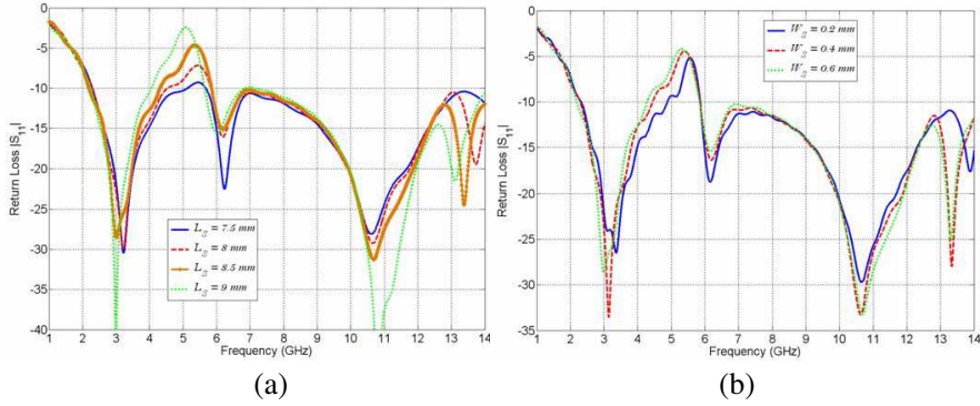
Figure 5. Simulated reflection coefficient curves for different (a) slot lengths L_S with W_S = 0.65 mm and D_S = 18.6 mm, (b) slot widths W_S with L_S = 8.6 mm and D_S = 18.6 .
