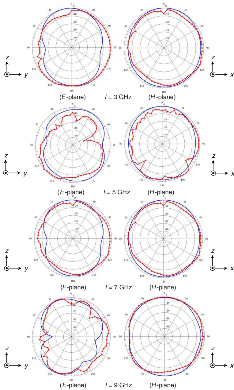
Figure 3. Measured (marker line) and calculated (solid line) radiation patterns of the proposed maple-leaf shaped printed monopole antenna.
