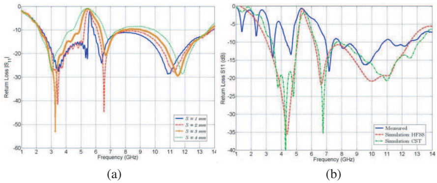
Figure 9. (a) Simulated reflection coefficient curves for different separation distance between slits S with L_S = 10.2 mm and W_S = 0.5 mm, (b) measured and simulated reflection coefficient curves for the proposed bandstop antenna using two slits.
