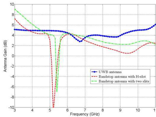
Figure 10. Gain curves versus frequency for the proposed antennas.
