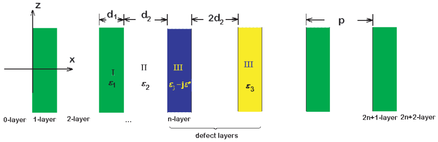
Figure 1. Configuration of the structure. The photonic crystal with defects is quarter-stack except the (n + 1) th layer, and the (n + 1) th layer's optical thickness is a half wavelength.
