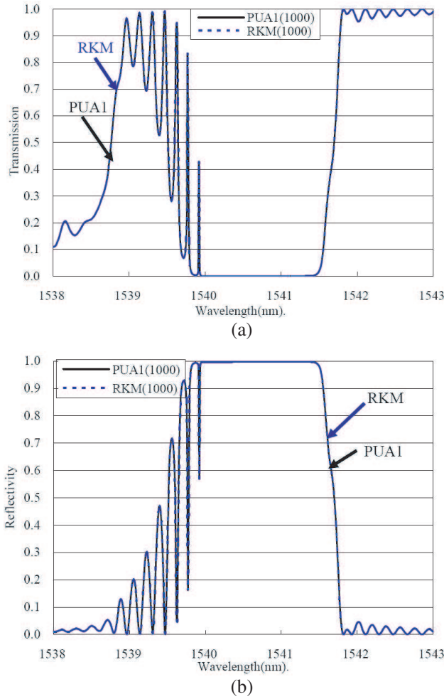
Figure 2. (a) The transmission spectrum of Gaussian-apodized gratings, (b) the reflection spectrum of Gaussian-apodized gratings. The solid line is calculated by PUA, the dash line is calculated by RKM.
