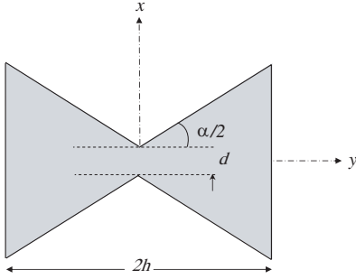
Figure 1. Geometry of bow-tie antenna.
