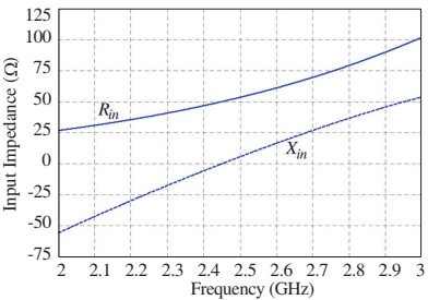
Figure 4. Input impedance versus frequency for an optimized bowtie antenna using BSO-NM ( h = 21.078 , d = 3.4818 , and \alpha = 48.555^\circ ).
