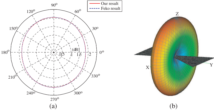
Figure 5. (a) A comparison between the resulting gain radiation pattern in x - z plane employing the MoM-based Feko technique and the results obtained via our program for optimized bow-tie antenna using BSO-NM ( h = 21.078 , d = 3.4818 , and \alpha = 48.555^\circ ) at 2.45 GHz. (b) 3D Radiation pattern for an optimized bowtie antenna using BSO-NM ( h = 21.078 , d = 3.4818 , and \alpha = 48.555^\circ ) at 2.45 GHz.
