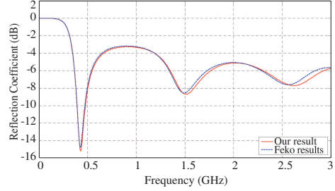
Figure 2. Reflection coefficient comparison between our result and Feko result for a bow-tie antenna ( h = 10 cm, d = 1 cm, and \alpha = 90^\circ ).
