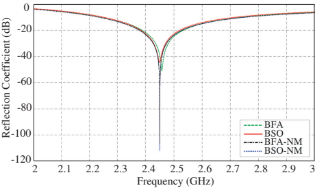
Figure 3. Reflection coefficient comparison for optimized bow-tie antenna using BFA, BSO, BFA-NM, BSO-NM algorithms.
