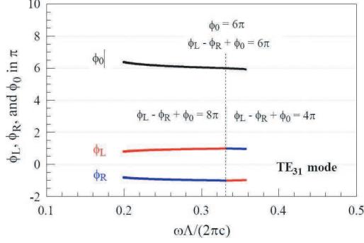
Figure A1. Profiles of \phi_L , \phi_R , and \phi_0 , and the transverse resonance conditions for \text{TE}_{31} mode with the mode order m = 3 and the band order n = 1 [21]. \phi_0 changes from 6.38\pi to 5.94\pi through 6\pi . \phi_L = -\phi_R except for at \phi_0 = 6\pi . At \phi_0 = 6\pi (dashed line), \phi_L = \phi_R = \pi , resulting from the discontinuity of the Fortran intrinsic function \text{DATAN2}(y, -1) at y = 0 . After the dashed line, \phi_L and \phi_R exchange the sign. Note: (i). On the left of the dashed line, \phi_L - \phi_R + \phi_0 = 8\pi with m_{TR} = 4 ; (ii). At \phi_0 = 6\pi , \phi_L - \phi_R + \phi_0 = 6\pi with m_{TR} = 3 ; (iii). On the right of the dashed line, \phi_L - \phi_R + \phi_0 = 4\pi with m_{TR} = 2 . The mode order m = 3 corresponds to three possible transverse resonance conditions with m_{TR} = 4, 3 , or 2 .
