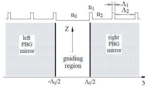
Figure 1. One-dimensional all-dielectric PBG light-guiding system, consisting of a guiding region and two symmetric half-infinite bilayer periodical structures. \Lambda_1 ( > 0 ) and \Lambda_2 ( > 0 ) are, respectively, the thickness of the first and second layers; n_1 and n_2 are their corresponding refractive indices. The structure period is \Lambda = \Lambda_1 + \Lambda_2 , and the width and refractive index of guiding region are, respectively, \Lambda_0 and n_0 .
