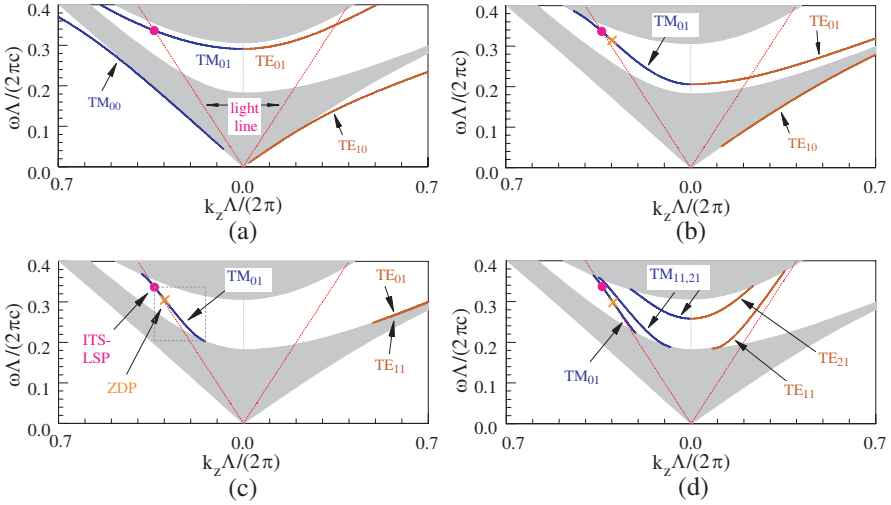
Figure 2. Evolution of mode structure with increase of the width of guiding region. Left side of the k_z = 0 line: TM mode; right side: TE mode; k_z > 0 for the both sides. White: Stop band; gray: Allowed band. Periodic structure's parameters: n_1 = 4.6 , n_2 = 1.6 ; \Lambda_1 = 0.3 \mu\text{m} , \Lambda_2 = 2.15 \mu\text{m} ; guiding region refractive index: n_0 = 1 . (a) \Lambda_0 = 0.02 \mu\text{m} ( 0.008\Lambda ), (b) \Lambda_0 = 1 \mu\text{m} ( 0.41\Lambda ), (c) \Lambda_0 = 3.6 \mu\text{m} ( 1.47\Lambda ), and (d) \Lambda_0 = 9.8 \mu\text{m} ( 4\Lambda ). The thickness ratio of the two layers is taken so that the intrinsic light-speed point (ITS-LSP, solid circle) is reasonably close to the top boundary of the first stop band to improve the bandwidth of single-mode guidance. The zero-dispersion point (ZDP, cross) shifts towards the low frequency side with the increase of the guiding region width \Lambda_0 . The dashed box in (c) shows the reflector-band single-mode regime. Properties of mode structure in the PBG reflector's band of the main first stop band: (i). Only the fundamental \text{TM}_{01} and \text{TE}_{01} modes exist when \Lambda_0 is small as seen in (a) and (b); (ii). Every pair of guided TM and TE modes is born with the same frequency at k_z = 0 (degeneration point); (iii). The fundamental \text{TE}_{01} mode completely disappears when \Lambda_0 is large enough as seen in (d) — Called “mode-lost phenomenon”; (iv). All PBG-guided mode curves shift down towards the low-frequency side as \Lambda_0 increases.
