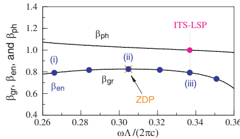
Figure 3. Normalized-to-vacuum-light-speed group velocity \beta_{gr} , energy velocity \beta_{en} , and phase velocity \beta_{ph} for the fundamental TM_{01} mode in single-mode regime. Sample \beta_{en} -points calculated from light-field distributions excellently fit the \beta_{gr} -curve. (i)- and (iii)-points have the same group velocity. (ii)-point overlaps the zero-dispersion point ZDP.
