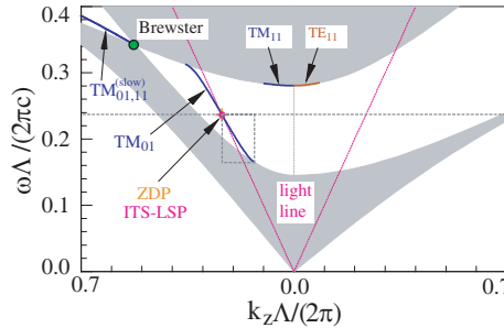
Figure 5. Mode structure for the planar bilayer PBG guiding system with a full-band single-mode regime. All parameters are the same as the ones in Fig. 2(c) except for the bilayer-unit-cell thickness ratio \Lambda_1/\Lambda_2 , which is increased to 0.6/1.85 here. The dashed box shows the full-band single-mode regime, and the intrinsic light-speed point (ITS-LSP) overlaps the zero-dispersion point (ZDP). There are two nearly-overlapping slow-wave modes below the Brewster's line (not drawn), labeled by \text{TM}_{01,11}^{(\text{slow})} . The main first TM stop band is defined as the band part between the Brewster's point and the k_z = 0 line. It can be intuitively seen that, if the light line were not located above the Brewster's line, then the light line would not pass through the main first TM stop band and there would be no intrinsic light-speed point within the main first TM stop band.
