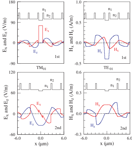
Figure 7. Field distributions of the fundamental TM_{01} and TE_{01} modes at light-speed points in two different kinds of planar light-guiding systems. The system's parameters are the same as the ones of Fig. 2(b) and Fig. 6, respectively. The TM_{01} mode of the 1st kind of guiding system and the TE_{01} mode of the 2nd kind are TEM field distributions in the guiding region. E_x -components of the 1st and 2nd kinds have opposite parities, and so do H_x -components.
