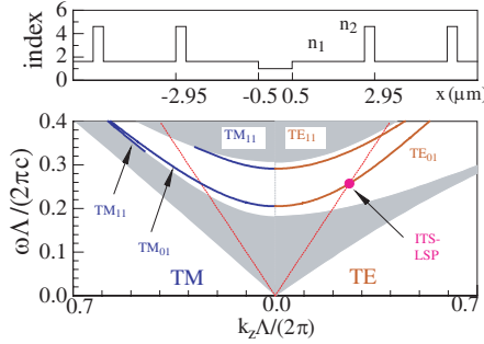
Figure 6. Mode structure for the second kind of planar light-guiding system that has exactly the same parameters as in Fig. 2(b), except for the index arrangement. The TE_{01} mode has an intrinsic light-speed point (ITS-LSP) instead. Compared with Fig. 2(b), this guiding system has a smaller mode separation, with TM_{11} (above TM_{01} ) and TE_{11} (above TE_{01} ) coming out from the top boundary and closely following TM_{01} and TE_{01} . On the bottom boundary, there is an emerging all-slow-wave TM_{11} (below TM_{01} ) and it will disappear when the guiding region width increase further. Note: the first and second kinds of planar light-guiding systems have the same band structure.
