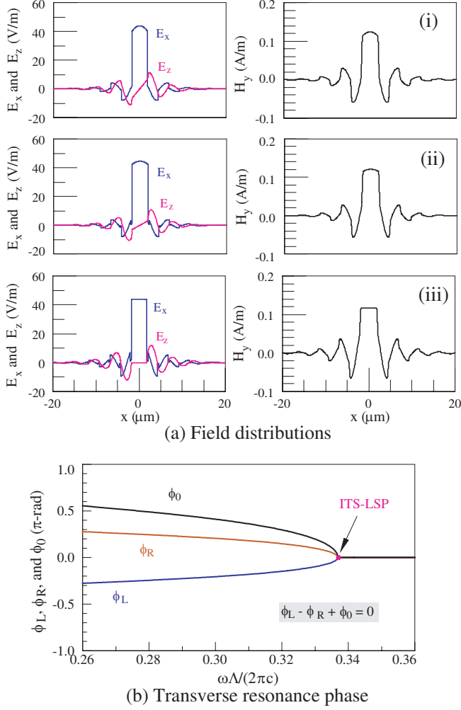
Figure 4. Field distributions and transverse resonance phase. (a) Distributions of electric and magnetic fields at points (i), (ii), and (iii) in Fig. 3. It is seen from (iii) that the fundamental \text{TM}_{01} mode at the intrinsic light-speed point (ITS-LSP) is a TEM field distribution in the guiding region. (All fields are drawn for a 10 \mu\text{W}/\text{m} flowing power.) (b) PBG mirror reflection coefficient arguments \phi_L and \phi_R , and round-trip phase shift \phi_0 for the \text{TM}_{01} mode in single-mode guidance regime. Note: \phi_L and \phi_R = -\phi_L vary with frequency, signifying the dispersion property of PBG mirrors.
