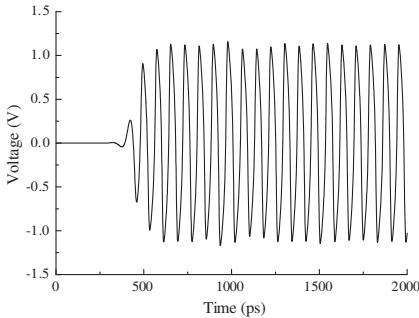
Figure 7. Time development of the total voltage across the diode D_1 when the quasi-ideal packaged diode model is used.
