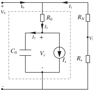
Figure 6. Equivalent circuit model of the loaded Gunn diode.
