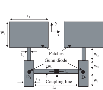
Figure 5. Layout of the two-element patch antenna.
