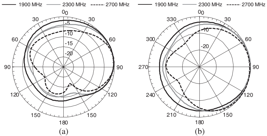
Figure 7. The radiation patterns of the proposed antenna at the frequencies 1900, 2300 and 2700 MHz for the principal planes: (a) E -plane, (b) H -plane.
