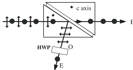
Figure 13. Glan type polarization prism with a HWP.
