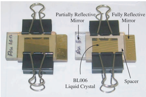
Figure 15. Two fabricated GTI LC cavities.
