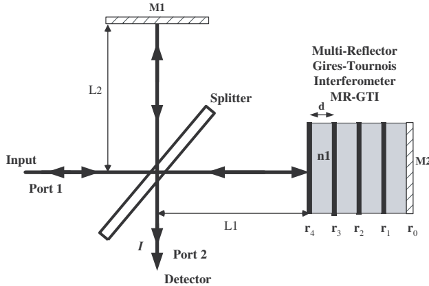
Figure 1. Michelson interferometer with a 5-reflector Gires-Tournois in one of the arms.
