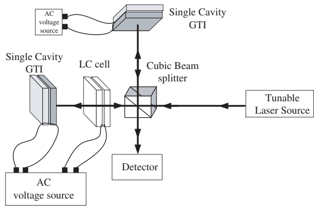
Figure 14. Experimental setup of the optical LC tunable interleaver.
