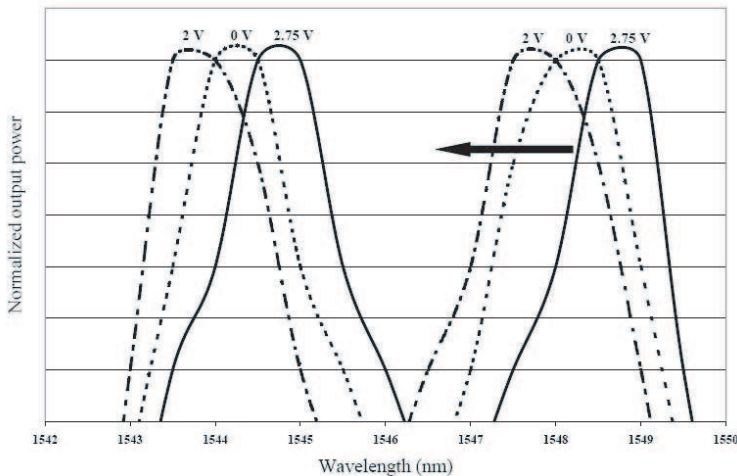
Figure 16. Measured channel tuning for different applied voltage values.
