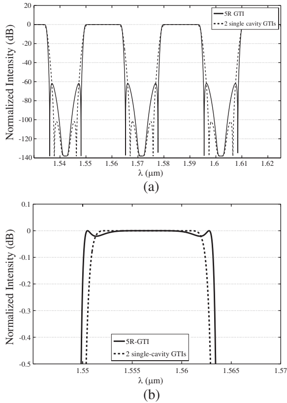
Figure 6. (a) Normalized output intensity for a combined MI with two single-cavity GTIs, and with MR-GTI (5 reflectors are used here) and (b) a close up of the -0.5 dB bandwidth.
