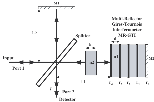
Figure 3. A combined Michelson interferometer with a multi-reflector Gires-Tournois with a liquid crystal cell to provide tunable phase delay.
