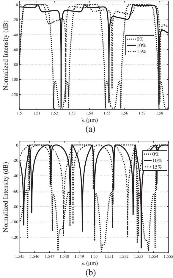
Figure 9. (a) Normalized output intensity for a combined MI with two single-cavity GTIs with GTI cavity thickness, d , 10 and 15% error. (b) For combined MI-5RGTI.
