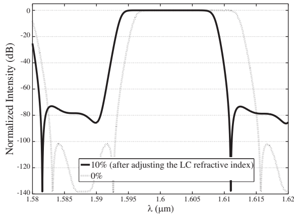
Figure 10. Normalized output intensity for a combined MI with two single-cavity GTIs after compensating the 10% GTI cavity thickness, d , error.
