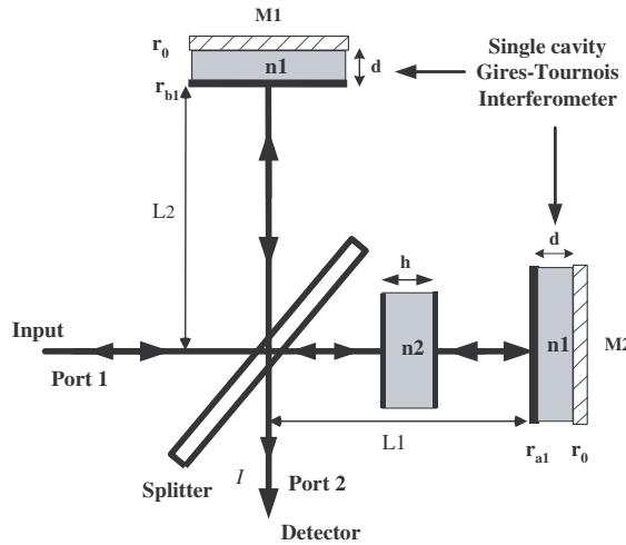
Figure 5. A combined Michelson interferometer with two single cavity Gires-Tournois with a liquid crystal to provide tunable phase delay.
