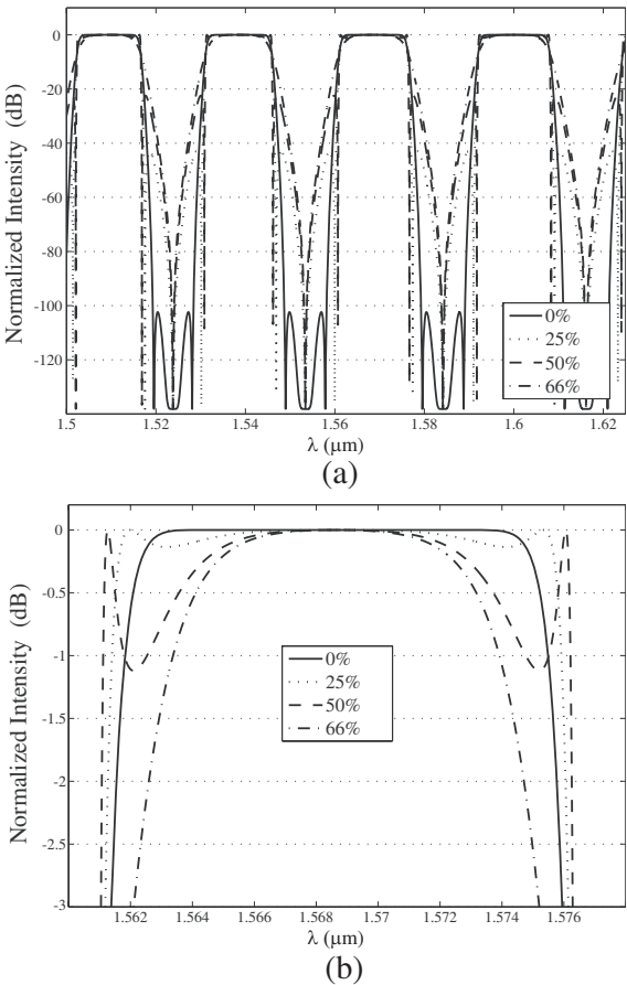
Figure 7. (a) Normalized output intensity for a combined MI with two single-cavity GTIs with reflection coefficients error. (b) A close up of the -3 dB bandwidth.
