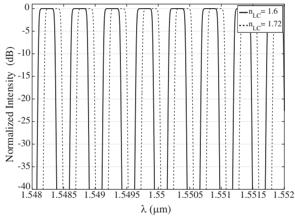
Figure 4. The normalized output intensity for the tunable interleaver for two different values of the LC refractive index.
