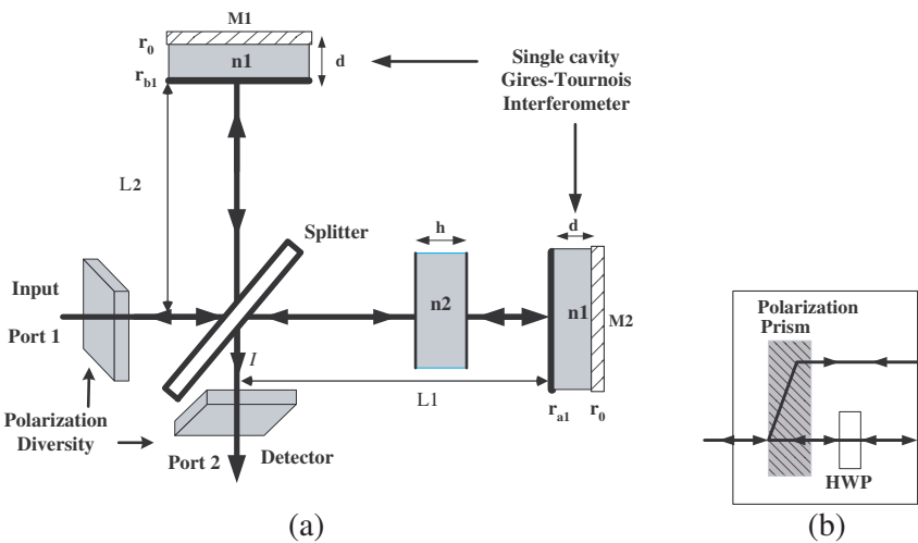
Figure 12. (a) A combined MI with two single cavity GTIs with a liquid crystal to provide tunable phase delay with polarization diversity and (b) polarization diversity device.
