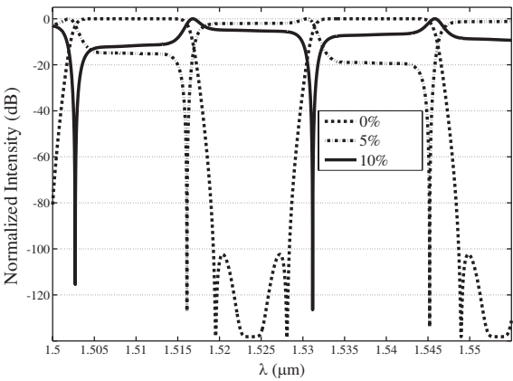
Figure 11. Normalized output intensity for a combined MI with two single-cavity GTIs with \Delta L has 5 and 10% error.
