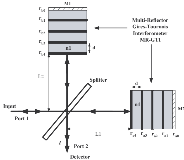
Figure 2. Michelson interferometer with two multi-cavity Gires-Tournois in the two arms with N = M = 5 .
