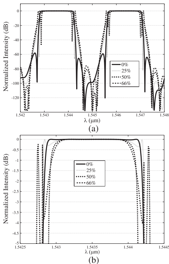
Figure 8. (a) Normalized output intensity for a combined MI with one 4-cavity GTIs (5 reflectors) with reflection coefficients error. (b) A close up of the -5 dB bandwidth.
