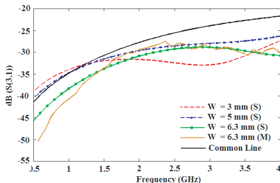
Figure 5. Simulated ( S ) and measured ( M ) crosstalk, S_{31} , of the common lines and stepped transmission lines for various first step widths W_1 . ( W_0 = 5 mm, W_2 = 3 mm, L = 6 mm).
