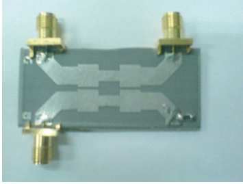
Figure 2. The photograph of the fabricated stepped-shaped transmission lines.
