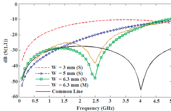
Figure 8. Simulate ( S ) and measured ( M ) Return loss, S_{11} , of a common line and new coupled line for various first step width W_1 . ( W_0 = 5 mm, W_2 = 3 mm, L = 6 mm).
