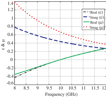
Figure 5. The real and imaginary parts of \epsilon , \mu versus frequency.
