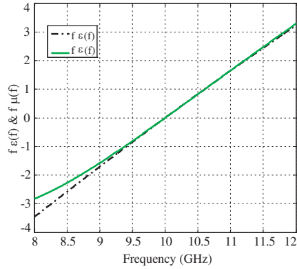
Figure 6. Variation of f\epsilon(f) , & f\mu(f) versus frequency for the Drude and Lorentz dispersion relations in Eq. (21) with parameters in Eq. (23).
