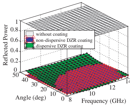
Figure 8. 3-D diagram of reflected power from a PEC plane versus frequency and angle of incidence under oblique incidence of a TM plane wave for three cases: (a) without coating. (b) With two layers of nondispersive DZR metamaterial coatings with characteristics given in Eq. (28). (c) With two layers of dispersive DZR metamaterial coatings with characteristics given in Eq. (29).
