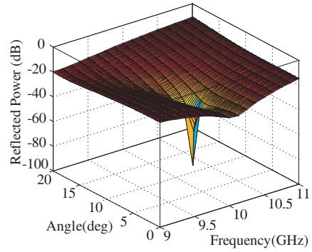
Figure 3. 3-D diagram of reflected power (in dB) from the structure in Fig. 1(a) with characteristics given in example 2 versus angle of incidence and frequency for TE polarization.
