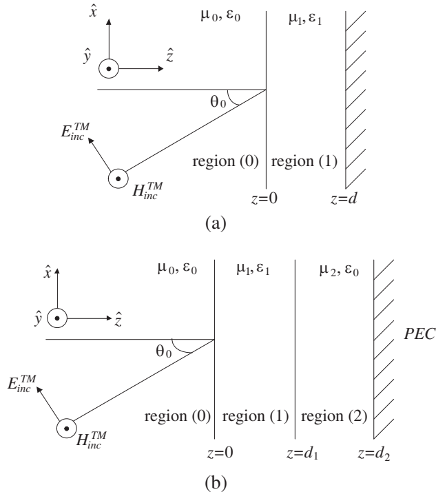
Figure 1. A perfect electric conducting (PEC) plate covered by DZR metamaterial layers.
