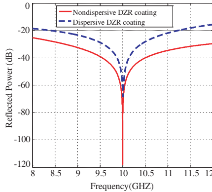
Figure 4. Reflected power (in dB) from the structure in Fig. 1(a) with characteristics given in example 3 versus frequency for normal incidence ( \theta_0 = 0^\circ ) for two cases: (a) Nondispersive DZR coating with characteristics in example (3), (b) dispersive DZR coating with parameters given in Eq. (23).
