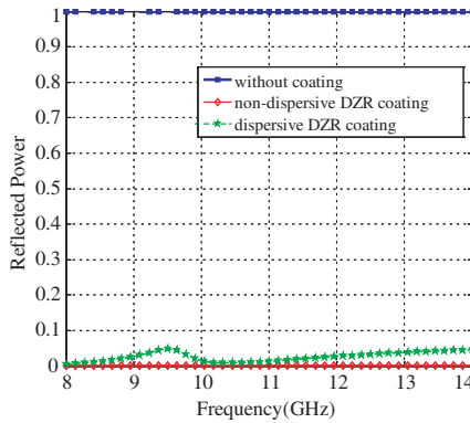
Figure 7. Reflected power from a PEC plane versus frequency (a) without coating (b) with two layers of nondispersive DZR metamaterial coatings with characteristics given in Eq. (26), (c) with two layers of dispersive DZR metamaterials with characteristics given in Eq. (27).
