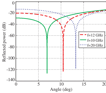
Figure 2. Reflected power (in dB) from the structure in Fig. 1(a) with characteristic given in example 1 versus the angle of incidence at frequencies f = 12 , 10, 20 GHz for TE polarization.
