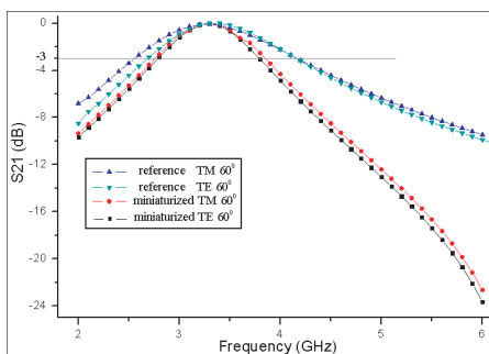
Figure 3. Transmission characteristics of the miniaturized FSS and the reference FSS for TE60° and TM60°.
