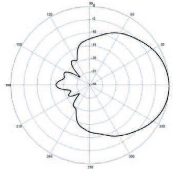
Figure 2. Radiation pattern of E_\theta for single element.
