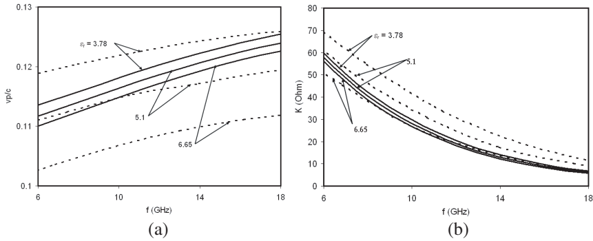
Figure 5. Comparison of theoretical (solid line) and simulated (HFSS) (broken line) phase velocity (a) and interaction impedance (b) versus frequency characteristics, taking the tip of the segment as the parameter.
