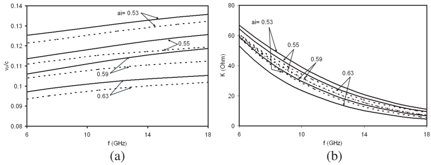
Figure 4. Comparison of theoretical (solid line) and simulated (HFSS) (broken line) results for the phase velocity (a) and interaction impedance (b) versus frequency characteristics, taking the helix inner radius ( a_i ) as the parameter.
