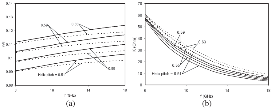
Figure 8. Comparison of theoretical (solid line) and simulated (HFSS) (broken line) phase velocity (a) and interaction impedance (b) versus frequency characteristics, taking the helix pitch as the parameter.
