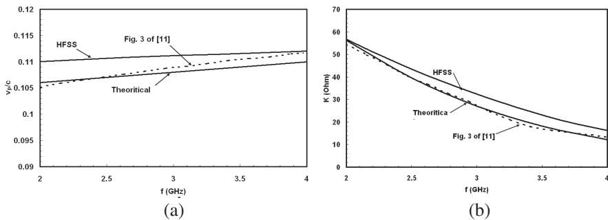
Figure 3. Comparison of dispersion characteristics (a) and interaction impedance (b) with the present analytical results, and the analytical results of Liu et al. [11] as well as with simulation (HFSS) values.
