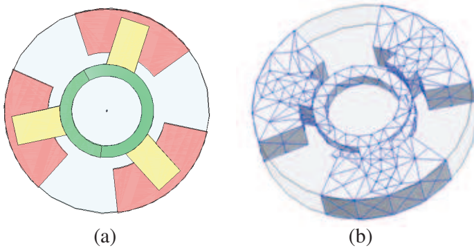
Figure 2. Simulation model of helical slow-wave structure (a) and with meshes (b).
