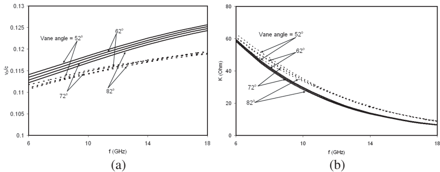
Figure 7. Comparison of theoretical (solid line) and simulated (HFSS) (broken line) phase velocity (a) and interaction impedance (b) versus frequency characteristics, taking the segment angle as the parameter.
