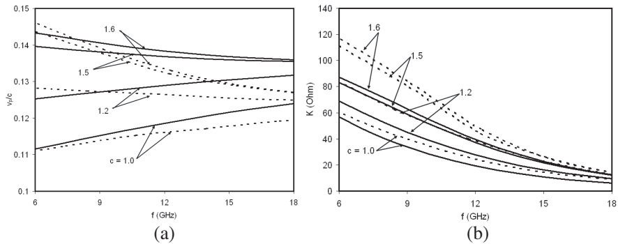
Figure 6. Comparison of theoretical (solid line) and simulated (HFSS) (broken line) phase velocity (a) and interaction impedance (b) versus frequency characteristics, taking permittivity of the support material ( \epsilon_r ) as the parameter.
