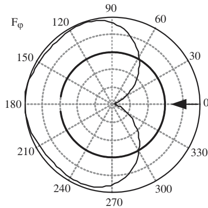
Figure 3. The distribution of F_\varphi(\varphi) in the far field ( k\rho = 2000 ). \varphi_0 = 0 , L_e = 1.15 (geometry of the structure is shown directly on the plot).
