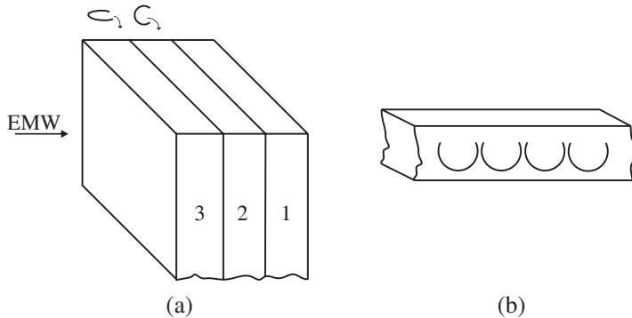
Figure 4. Low reflecting coating structure (a) and direct box with a dielectric array in the form of identically oriented flat open rings on one of its surfaces (b). 1 — absorber, 2 — layer composed of vertically glued dielectric parallelepipeds, 3 — layer that composed of horizontally bonded dielectric parallelepipeds (b).
