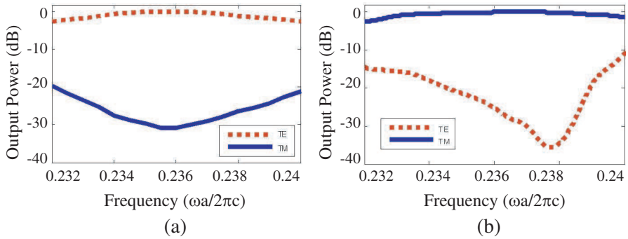
Figure 5. The output powers from the two output ports varies with the wavelength for both polarizations (a) Port 3; (b) Port 2.
