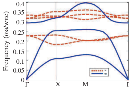
Figure 3. The band diagrams of the internal PhC section. The dotted and solid lines represent the polarization bands of TE and TM polarizations, respectively.
