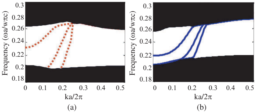
Figure 2. The projected band diagram for the W6 PhC waveguide for (a) TE polarization; (b) TM polarization.
