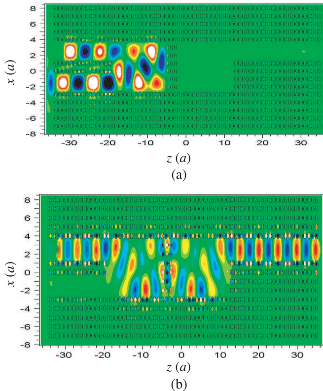
Figure 4. FDTD simulation for the field distribution at frequency f = 0.236(2\pi c/a) in the present PBS (a) TE Polarization; (b) TM Polarization.
