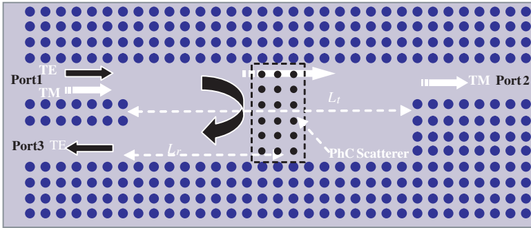
Figure 1. The schematic configuration of the proposed PBS.
