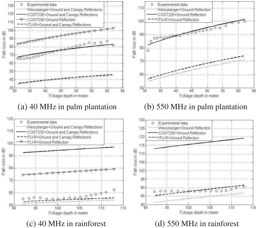
Figure 3. Measured and predicted path loss at VHF and low UHF bands with h_1 = 6.85 m and h_2 = 2.15 m in the palm plantation, and h_1 = 4.65 m and h_2 = 2.15 m in the rainforest.
