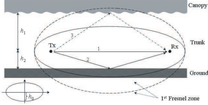
Figure 1. Ray tracing geometry of the direct — 1, ground-reflected — 2, and tree-canopy-reflected — 3 waves.
