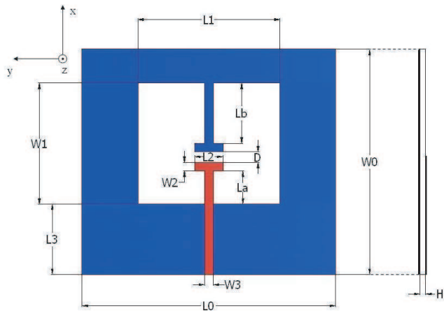
Figure 1. Geometry of the proposed antenna.
