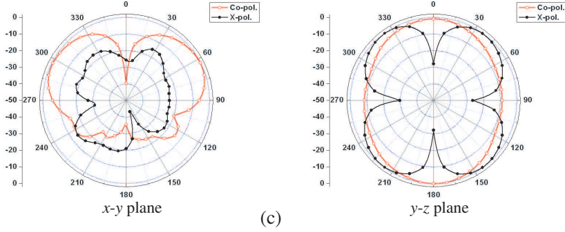
Figure 6. Measured radiation far-field patterns for the proposed antenna operating at (a) 2.4 GHz, (b) 5.2 GHz and (c) 5.8 GHz.
