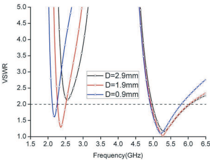
Figure 5. Simulated VSWR for different values of D ( R = 0.55 ).
