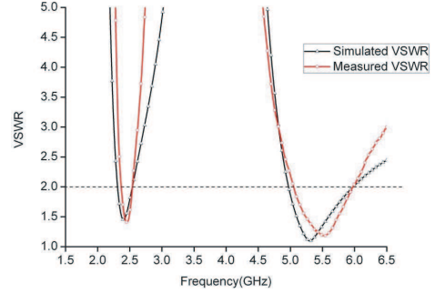
Figure 3. Simulated and measured VSWR of the proposed antenna with parameters R = 0.55 and D = 1.9 mm.
