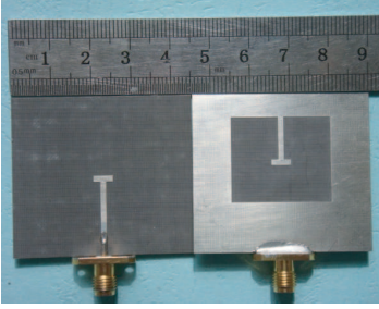
Figure 2. Prototype of the proposed antenna.
