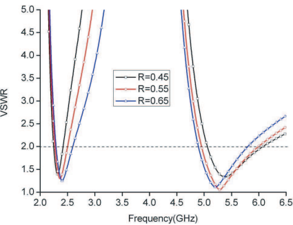
Figure 4. Simulated VSWR for different values of R ( D = 1.9 mm).
