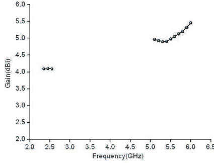
Figure 7. Measured peak gains of the proposed antenna.
