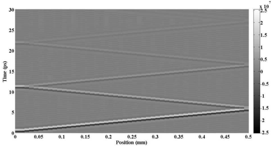
Figure 2. THz electric field inside the ZnTe slab as a function of time and space in the absence of the optical field.
