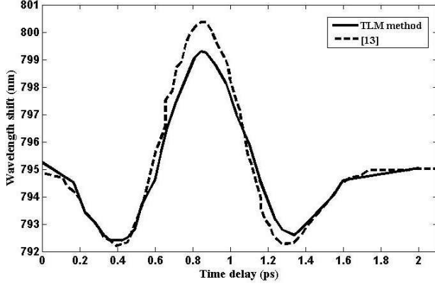
Figure 6. THz induced-wavelength shift of the optical beam versus the time delay between the THz and optical signal, the dashed-line curve corresponds to the result of [13] and the solid-line one shows the result of the TLM method.
