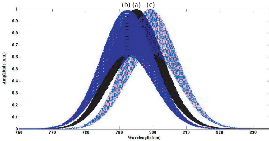
Figure 5. (a) Optical beam propagating in the ZnTe slab with no THz signal, (b) the blue shift corresponds to the case in which the input time delay is 0.3914 ps, (c) the red shift corresponds to the case in which the input time delay is 0.8418 ps.
