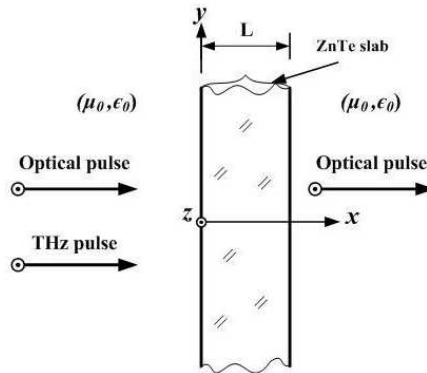
Figure 1. The optical and THz pulse in the form of a plane wave applied to the ZnTe slab covering 0 < x < L .
