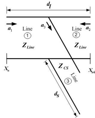
Figure 4. Transmission lines for the cell covering X_n < x < X_{n+1} . The change of the refractive index of ZnTe due to the THz pulse is modeled with the variation of the parameters of the shunt open stub.
