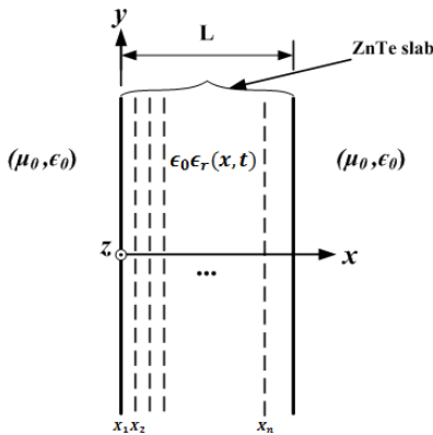
Figure 3. ZnTe slab is discretized by cells as small as a tenth of the optical wavelength. The relative permittivity of the slab varies as a function of space and time because of the THz pulse.
