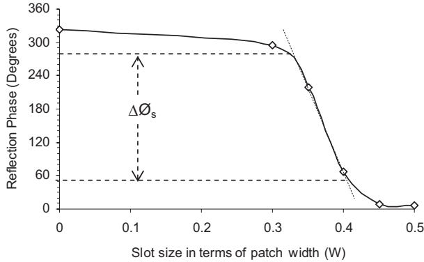
Figure 12. Measured phase shift versus slot size curve.
