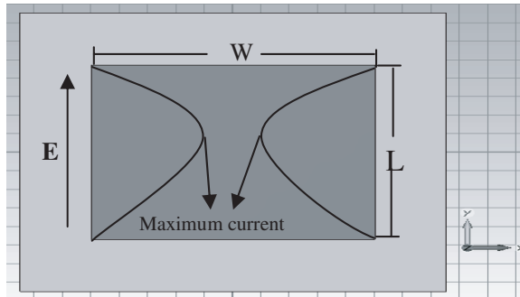
Figure 1. A reflectarray unit cell surface currents.
