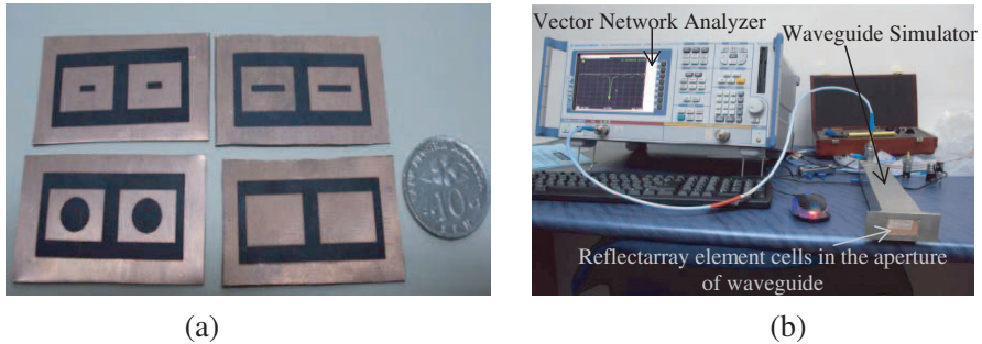
Figure 6. (a) Fabricated samples of reflectarrays with different slot configurations. (b) Measurement setup for scattering parameters measurements.
