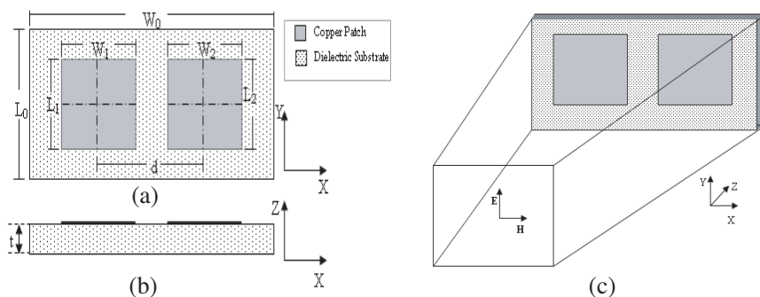
Figure 5. Geometry of two patch element reflectarray (a) top view and (b) side view (c) waveguide simulator for simulating an infinite array.
