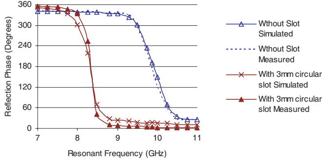
Figure 8. Simulated and measured reflection phase for 3 mm Circular slot.
