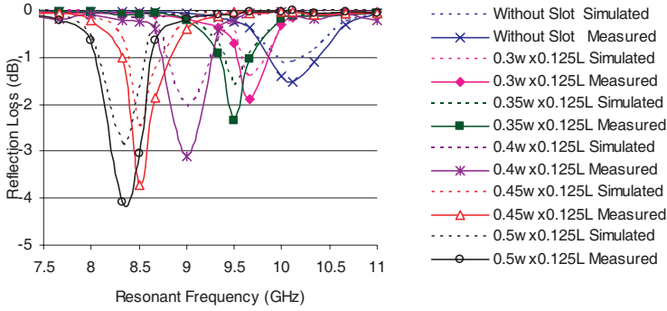
Figure 9. Simulated and measured reflection loss for different widths of rectangular slots.
