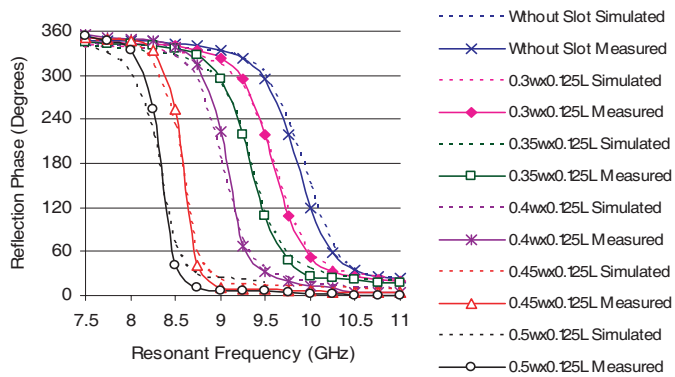
Figure 10. Simulated and measured reflection phase for different widths of rectangular slots.
