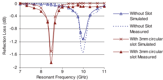
Figure 7. Simulated and measured reflection loss for 3 mm Circular slot.
