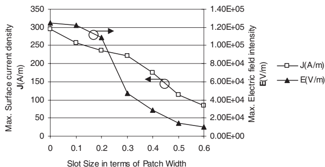
Figure 4. Maximum surface current and electric field intensity for different patch widths at resonant frequency.
