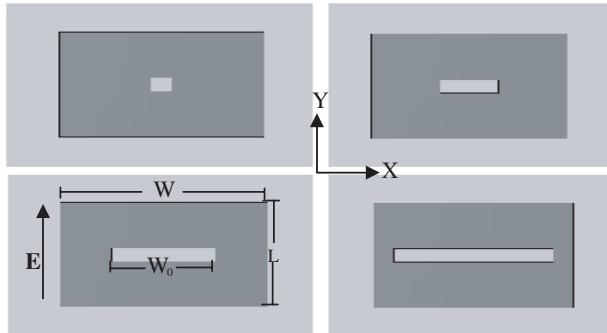
Figure 3. Rectangular slots with different widths in patch elements.
