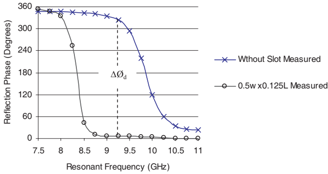
Figure 11. Dynamic phase range for 0.5W \times 0.125L rectangular slot.
