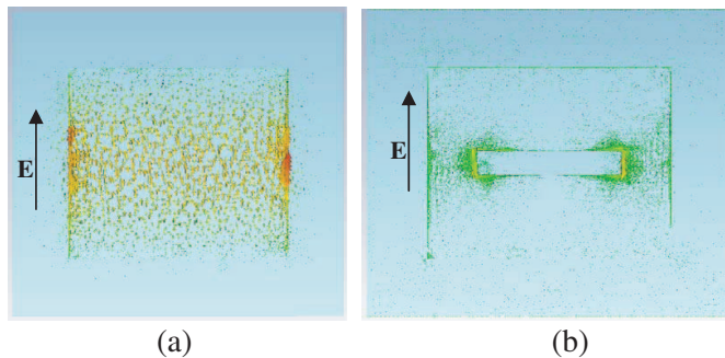
Figure 2. Surface current distribution on a patch element. (a) Without slot. (b) With a rectangular slot.
