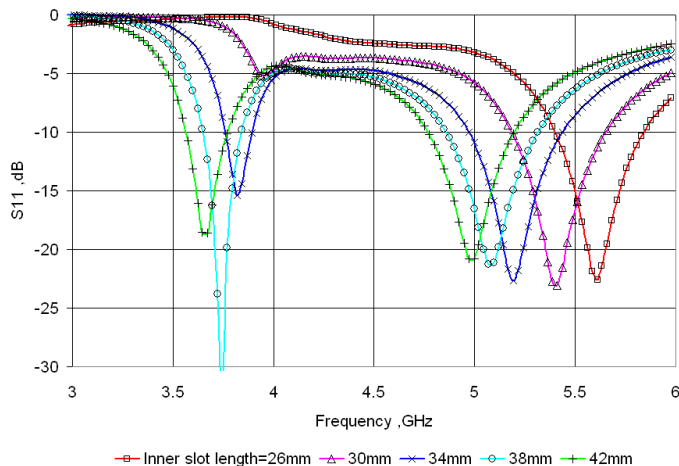
Figure 4. S_{11} variation as the total length of the inner slot is varied from 26 mm to 42 mm. Other dimensions of the antenna are in Table 1 [18].
