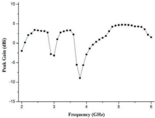
Figure 6. Gains of the antenna versus different frequencies.
