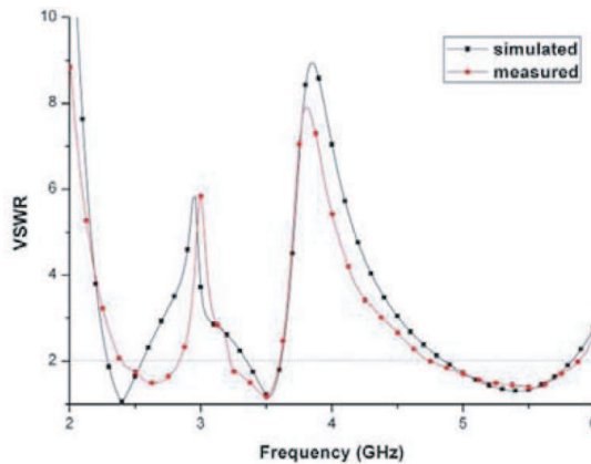
Figure 4. The measured and simulated VSWR of the antenna.
