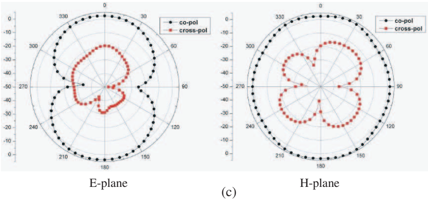
Figure 5. Radiation patterns of the proposed antenna at (a) 2.5 GHz, (b) 3.5 GHz and (c) 5.5 GHz.
