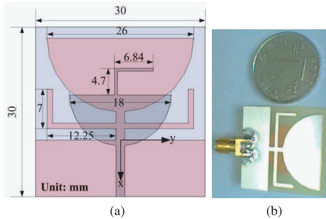
Figure 1. The (a) structure and (b) photograph of the proposed antenna.
