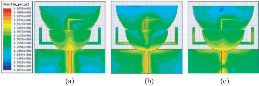
Figure 3. Current distribution at different frequencies (a) 2.5 GHz, (b) 3.5 GHz, (c) 5.5 GHz.
