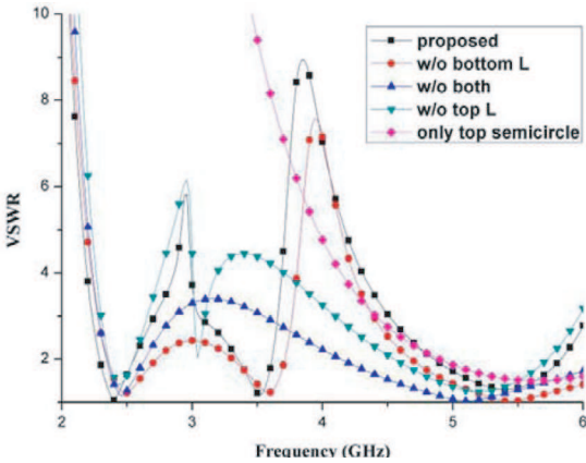
Figure 2. Simulated VSWRs of the antenna under different conditions.
