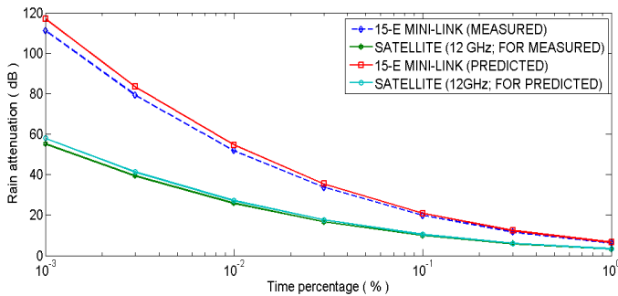
Figure 3. Comparison of terrestrial and satellite rain attenuation.
