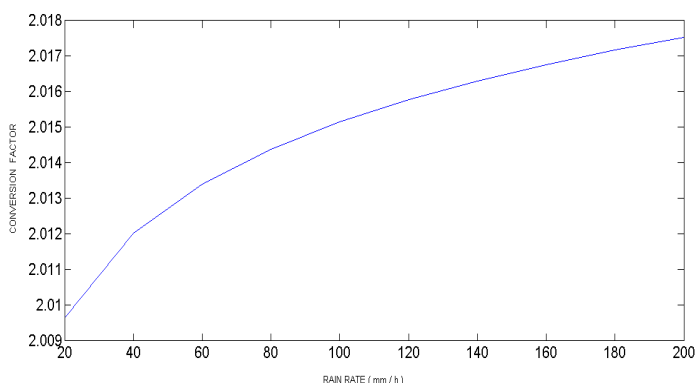
Figure 1. Variation of conversion factor with respect to rain rate.
