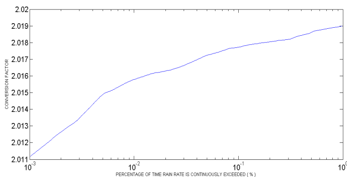
Figure 2. Variation of conversion factor with p\% of the time in an average year.
