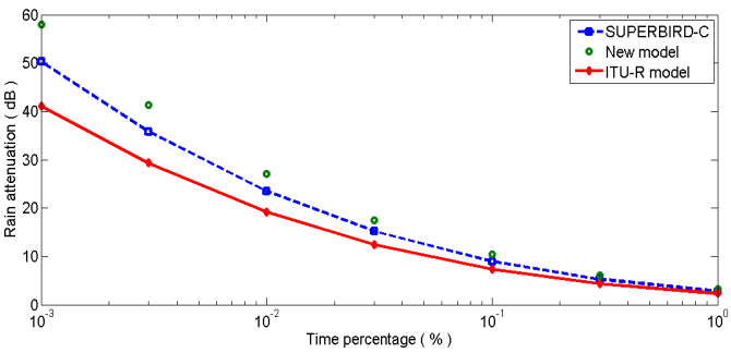
Figure 5. Comparison between measured and predicted attenuation for SUPERBIRD-C, USM.
