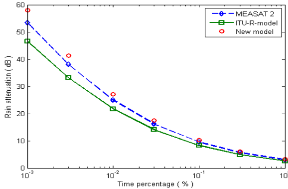
Figure 4. Comparison between measured and predicted attenuation for MEASAT 2-UTM.
