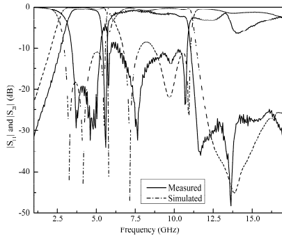
Figure 11. Simulated and measured frequency response.
