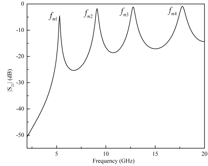
Figure 3. |S_{21}| of the initial MMR.
