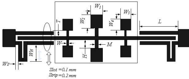
Figure 1. Schematic of the proposed UWB BPF.
