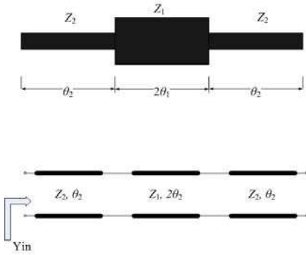
Figure 2. Geometry and the equivalent model of the initial MMR.
