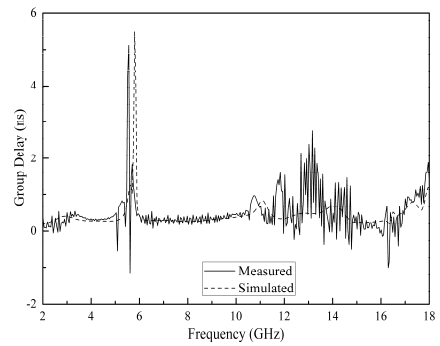
Figure 12. Simulated and measured group delay.
