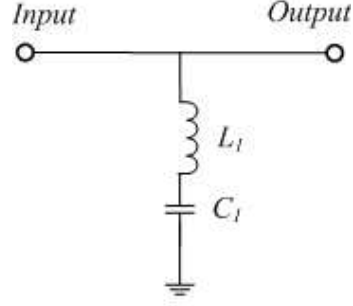
Figure 7. Equivalent circuit of the folded arm.
