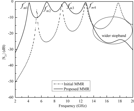
Figure 6. |S_{21}| comparison of initial and proposed MMR.
