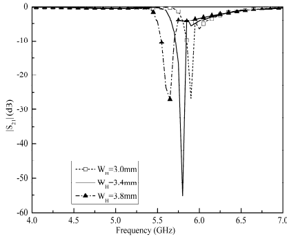
Figure 9. |S_{21}| response with varied W_H .
