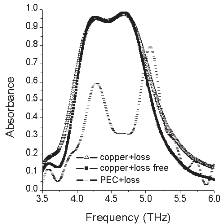
Figure 5. Simulated absorbances under three different loss conditions.
