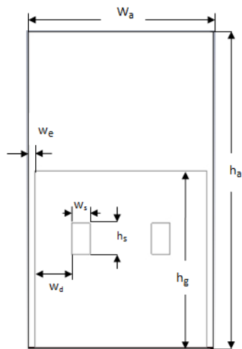
Figure 3. Back view of the proposed antenna.
