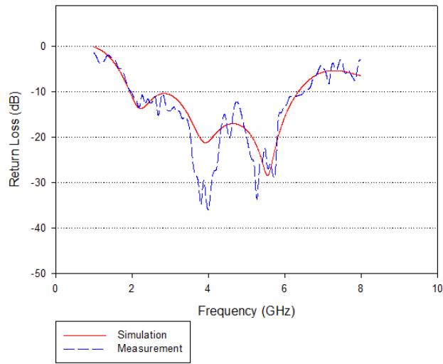
Figure 4. Simulated and measured return loss for UTM-Logo shape surrounded with ring patch antenna.
