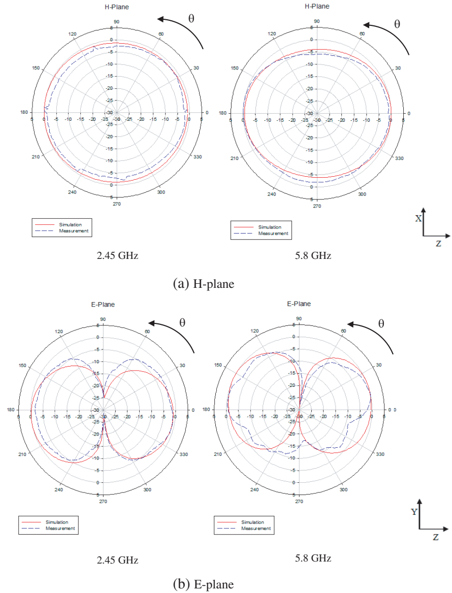
Figure 5. Simulated radiation pattern for UTM-Logo shape surrounded with ring patch antenna at 2.45 GHz and 5.8 GHz for (a) H -plane, (b) E -plane.
