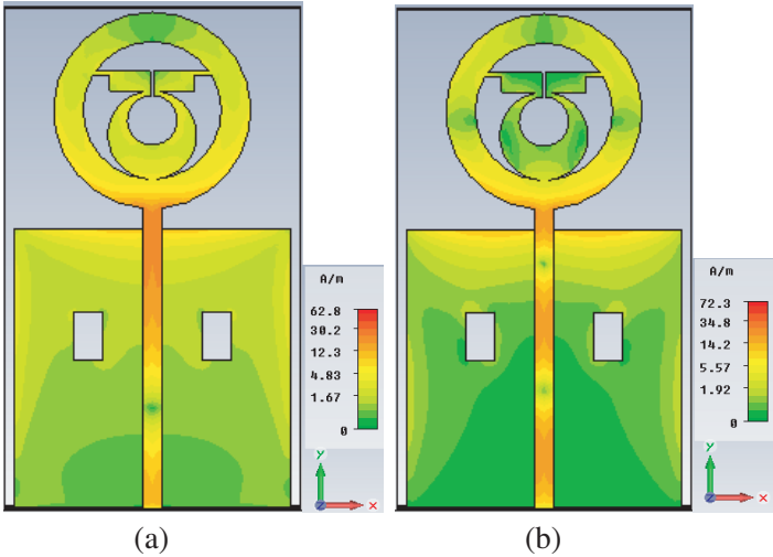
Figure 6. Current distribution for UTM-Logo shape surrounded with ring patch antenna at: (a) 2.45 GHz, (b) 5.8 GHz.
