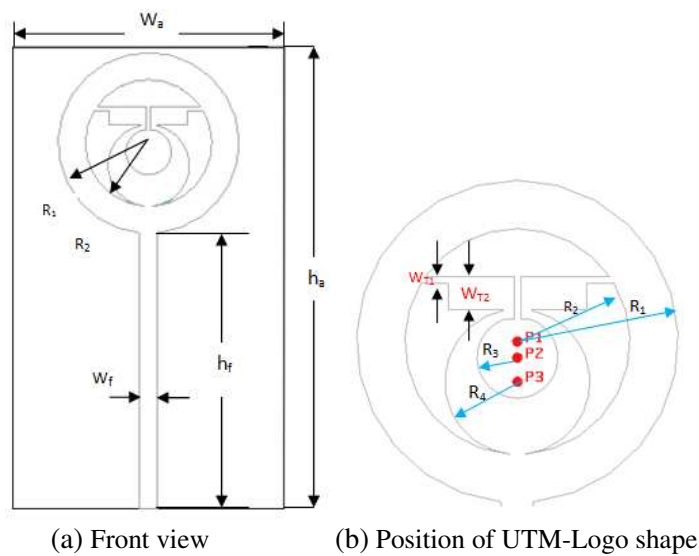
Figure 2. The geometry of the proposed UTM-Logo shaped antenna.
