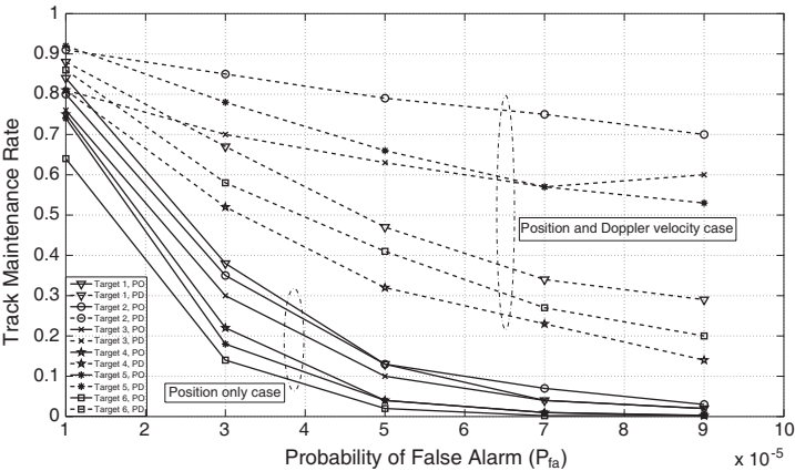
Figure 3. Track Maintenance Rate estimation of TAM unit for the benchmark targets and various P_{fa} values ( P_d = 0.80 ).
