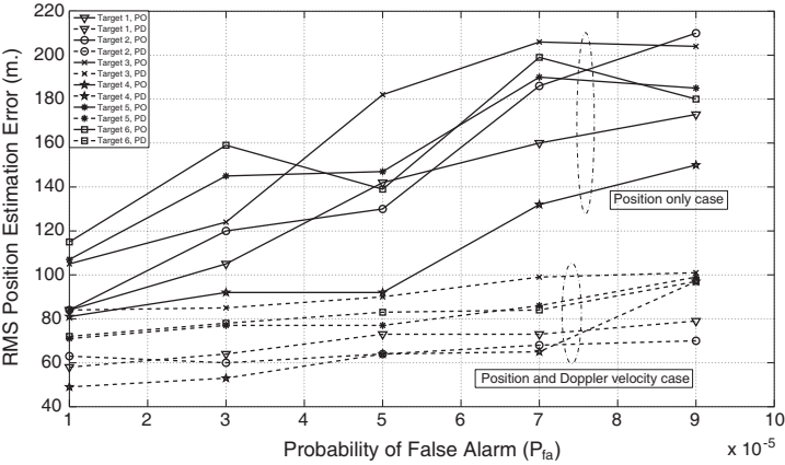
Figure 4. RMS Position Error estimation of TAM unit for the benchmark targets and various P_{fa} values ( P_d = 0.80 ).
